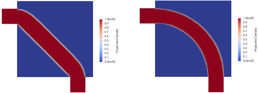
(A) Projected density field \bar{\gamma} : laminar-optimized topology ( Re = 1 ).
