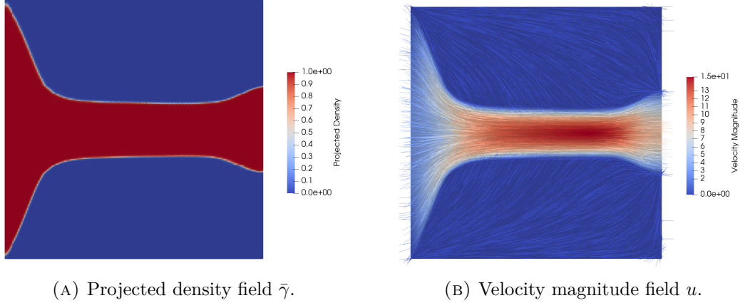
FIGURE 6.12: FEniCS-SA optimization result for the diffuser benchmark at V_f = 0.30 . Final objective function value J_D = 6.2274 \times 10^5 W/m.
