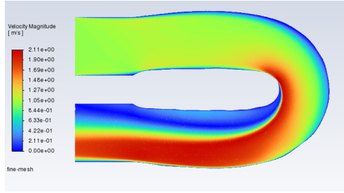
(A) SST velocity magnitude field u : laminar-optimized design.
