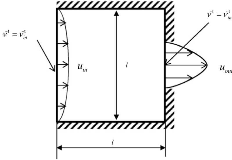
FIGURE 6.11: Geometry and boundary conditions for the diffuser benchmark from Yoon [47].
