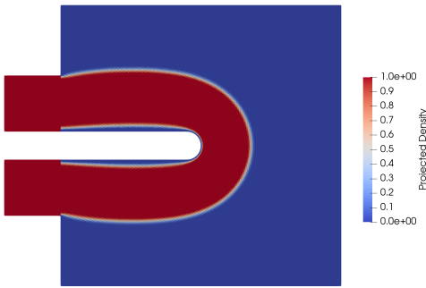
(A) Projected density field \bar{\gamma} : laminar-optimized U-bend topology ( Re = 1 ).
