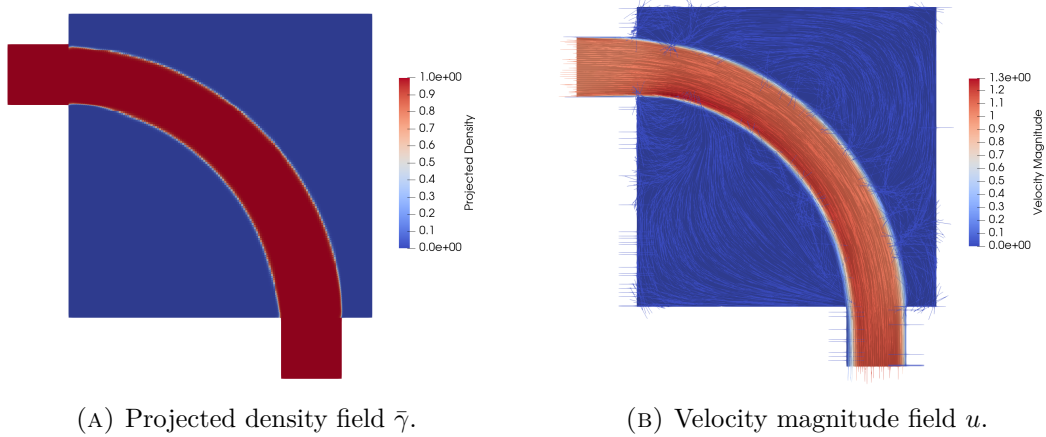
FIGURE 6.2: FEniCS-SA optimization result for the pipe-bend benchmark at V_f = 0.25 . Final objective function value J_p = 0.2032 Pa.
