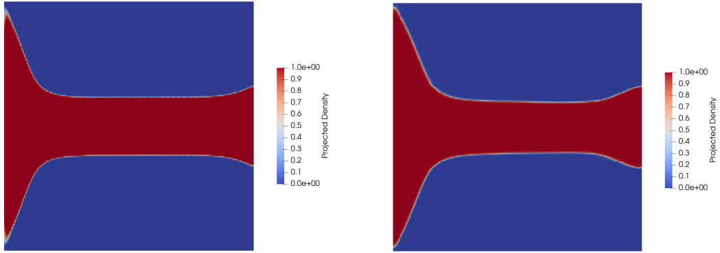
(A) Projected density field \bar{\gamma} : laminar-optimized diffuser topology ( Re = 1 ).
