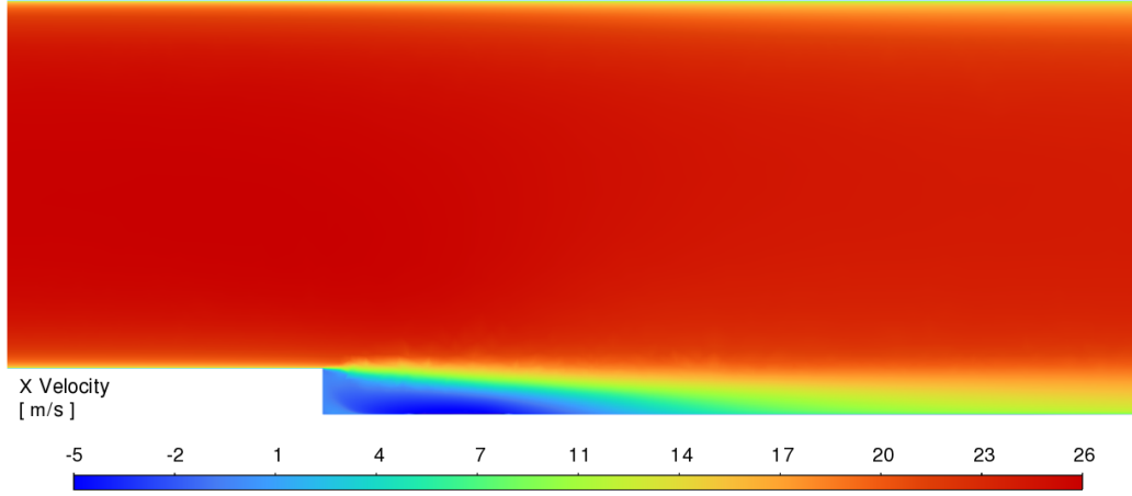
(A) SST k - \omega contour for u_x .
