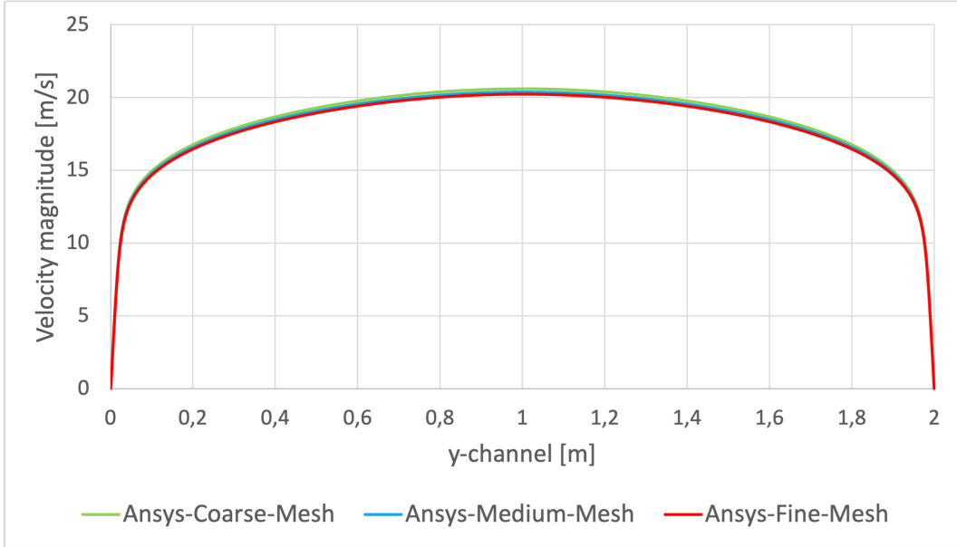
FIGURE A.2: Wall-normal velocity profiles extracted at x = 0.5L for the Coarse, Medium, and Fine grids in the Ansys periodic channel flow benchmark, demonstrating spatial convergence of the baseline data.
