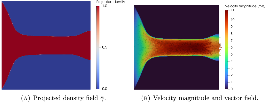
FIGURE 6.12: FEniCS-SA result for the velocity-outlet diffuser baseline at V_f = 0.30 . Final objective value J_D = 3.1164 \times 10^5 W/m.
