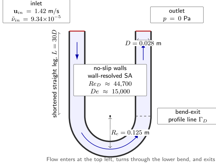
FIGURE 4.4: Schematic of the shortened 2D U-bend verification setup based on the VMFL048 operating point from the Ansys verification manual [8]. The profile line \Gamma_D is used for the bend-exit velocity comparison.
