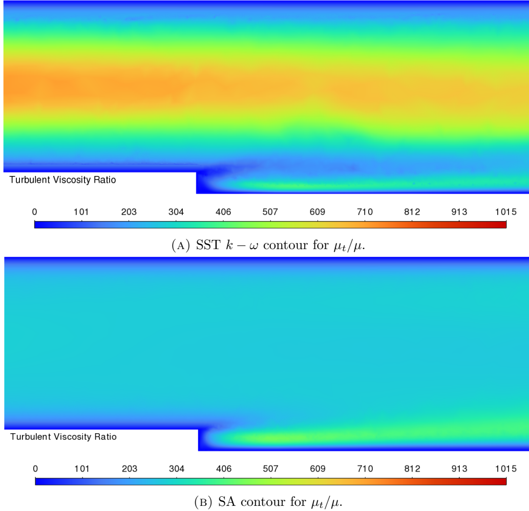
FIGURE 2.14: Turbulent-viscosity-ratio contours for the backward-facing-step benchmark, plotted with a common color scale. SA produces a smoother, more moderate eddy-viscosity field, while SST k - \omega gives a more stratified distribution with stronger variation between the near-wall/reverse-flow region and the outer shear-dominated flow.
