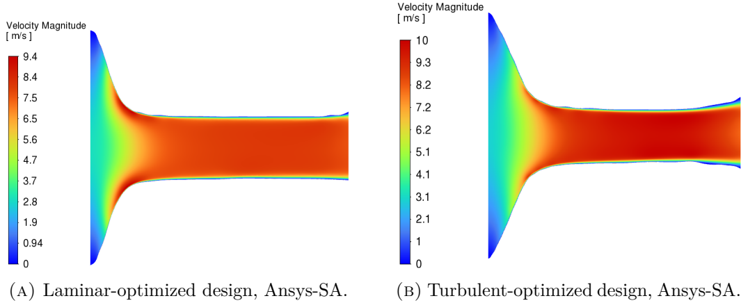
FIGURE 6.17: Ansys-SA velocity-magnitude comparison for the extracted pressure-outlet diffuser designs under identical turbulent operating conditions.
