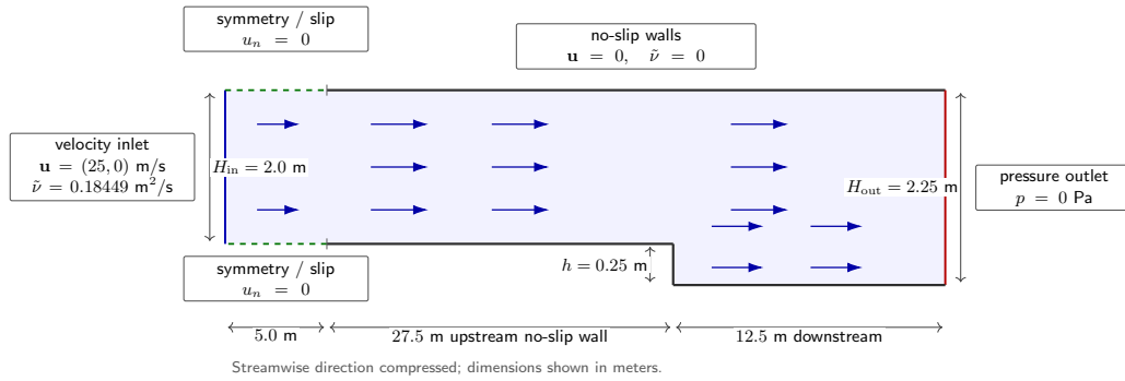
FIGURE 2.12: Backward-facing-step benchmark geometry and boundary conditions, based on the configuration used by Marcibál and the associated GitHub implementation [35, 30]. The first 5.0 m of the upper and lower boundaries are treated as symmetry/slip segments, while all remaining solid boundaries are no-slip walls. The streamwise dimension is compressed for readability.
