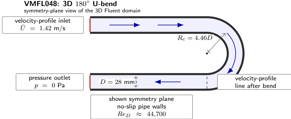
FIGURE 2.6: Geometry and boundary conditions for the VMFL048 3D U-bend benchmark adopted from the Ansys Fluid Dynamics Verification Manual [8]. The schematic is not to scale.
