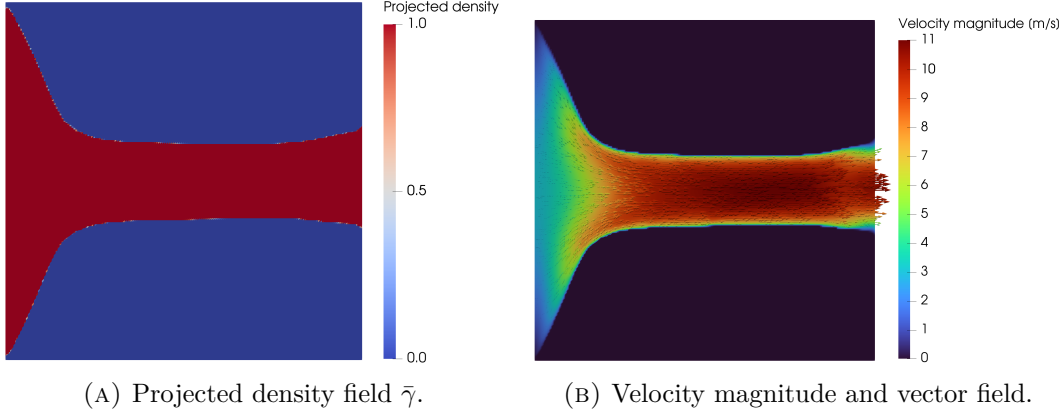
FIGURE 6.14: FEniCS-SA optimization result for the pressure-outlet diffuser at V_f = 0.30 . Final objective value J_D = 2.7664 \times 10^5 W/m.
