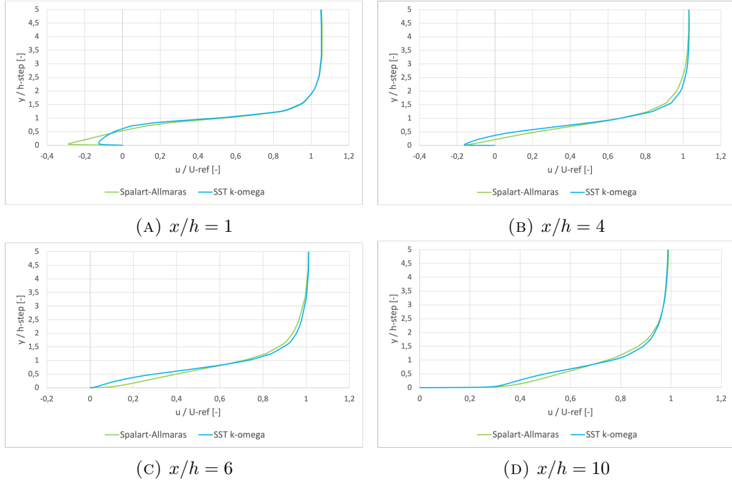
FIGURE 2.15: Normalized streamwise velocity profiles for the backward-facing-step benchmark at four downstream stations. The comparison isolates model-form sensitivity by running SA and SST k - \omega on the same sudden-expansion geometry and boundary conditions.
