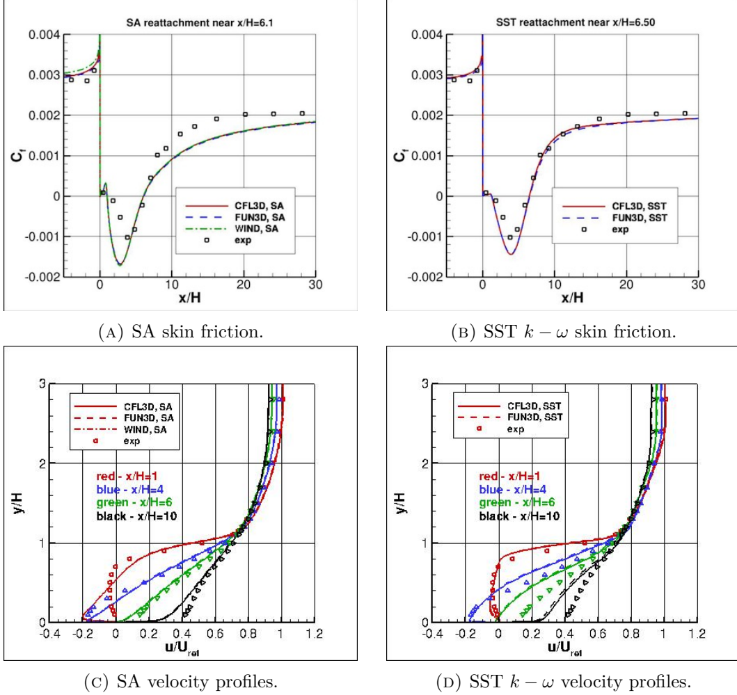
FIGURE 2.5: NASA Turbulence Modeling Resource comparison of SA and SST k - \omega predictions with the Driver-Seegmiller backward-facing-step experiment at Re_H \approx 36,000 [20, 38]. The skin-friction plots give the reattachment behavior, while the velocity profiles show the separated-flow recovery downstream of the step. The velocity-profile comparison indicates better agreement for SST k - \omega than for SA.
