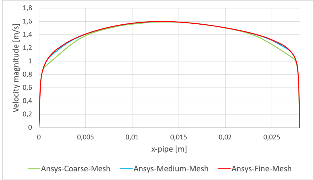
FIGURE A.4: Velocity profiles at the U-bend exit, extracted across the pipe diameter D = 0.028 m, for the Coarse, Medium, and Fine Ansys grids, demonstrating spatial convergence of the commercial baseline.
