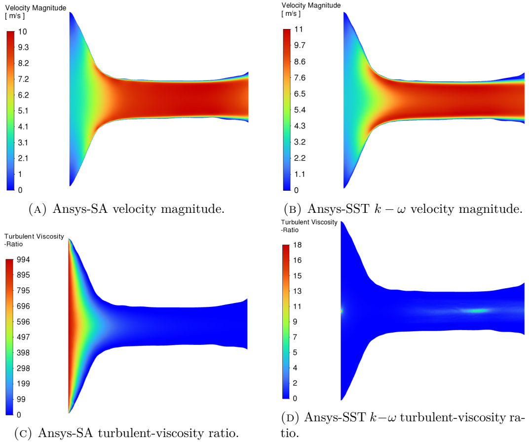
FIGURE 6.15: Closure diagnostics for the pressure-outlet turbulent diffuser. The velocity contours are similar enough that repeated full-domain velocity plots are not the main evidence; the turbulent-viscosity-ratio contours show the mechanism behind the much larger SA loss prediction.
