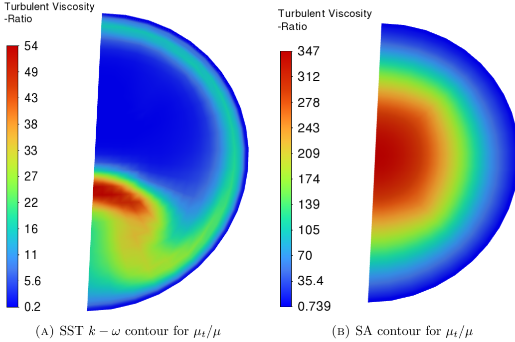
FIGURE 2.11: Turbulent-viscosity ratio contours for the VMFL030 90° pipe bend. Compared with SST k - \omega , SA predicts a much larger and more spatially uniform eddy-viscosity field across the section.
