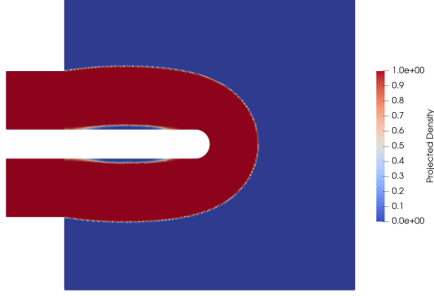
(A) Projected density field \bar{\gamma} : laminar-optimized design ( Re = 1 ). Final objective value J_p = 136.181 Pa.
