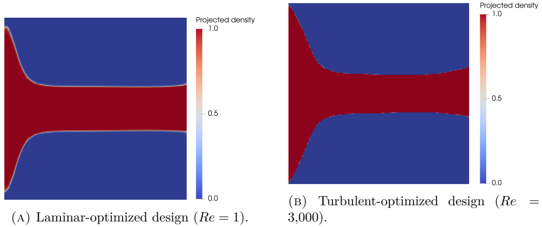
FIGURE 6.16: Laminar and turbulent topology comparison for the pressure-outlet diffuser benchmark.
