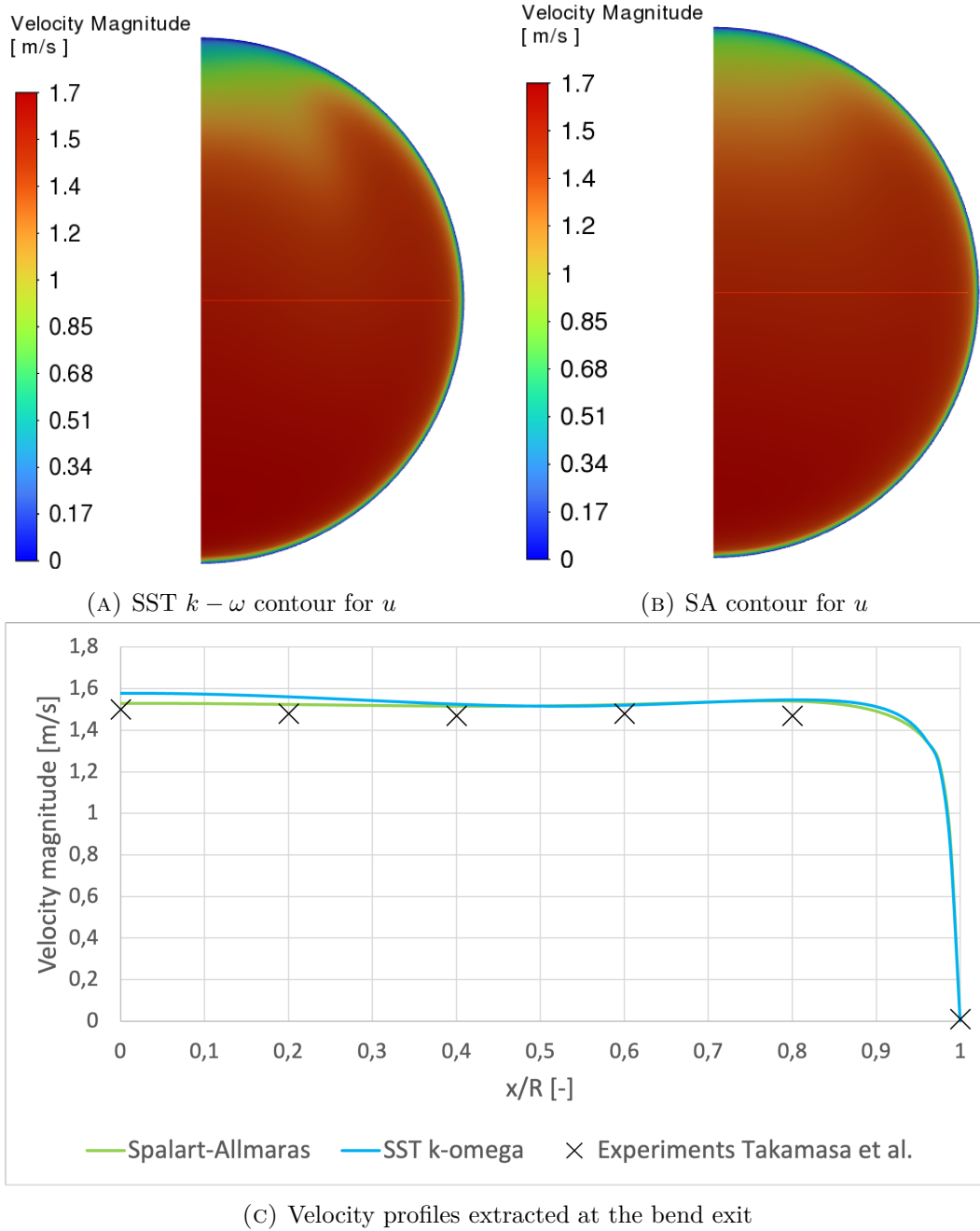
FIGURE 2.7: Flow predictions for the VMFL048 U-bend. Panels (a) and (b) show velocity contours with the radius used for profile extraction; panel (c) compares the resulting velocity profiles from x/R = 0 at the inner side of the pipe to x/R = 1 at the wall. The SA model matches the SST k-\omega contours and aligns with the experimental data from Takamasa and Kondo [55].
