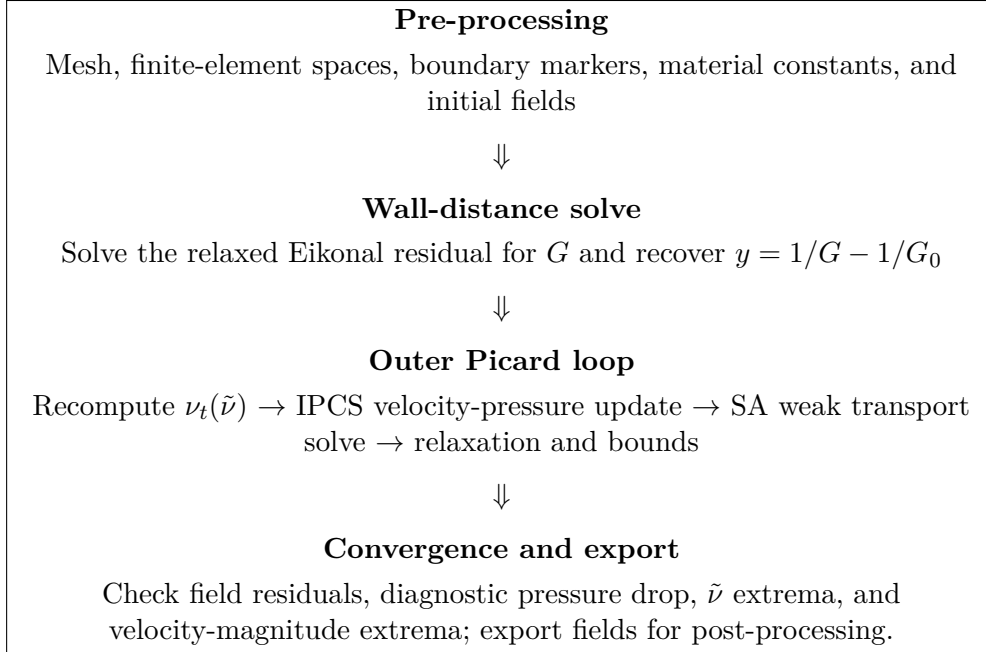
FIGURE 3.1: Algorithmic path of the standalone FEniCS RANS-SA verification solver. The wall distance is computed first, after which the segregated Picard loop alternates between IPCS flow solves and SA working-variable transport updates.
