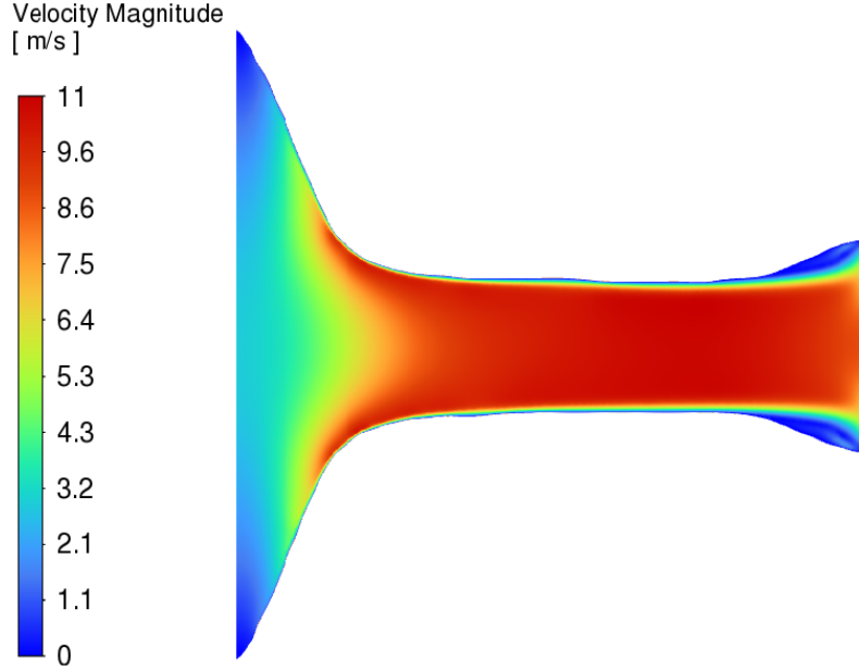
FIGURE 6.13: Ansys-SA velocity-magnitude contour for the extracted velocity-outlet diffuser baseline. The low-speed region near the widened outlet motivates the pressure-outlet sensitivity study.
