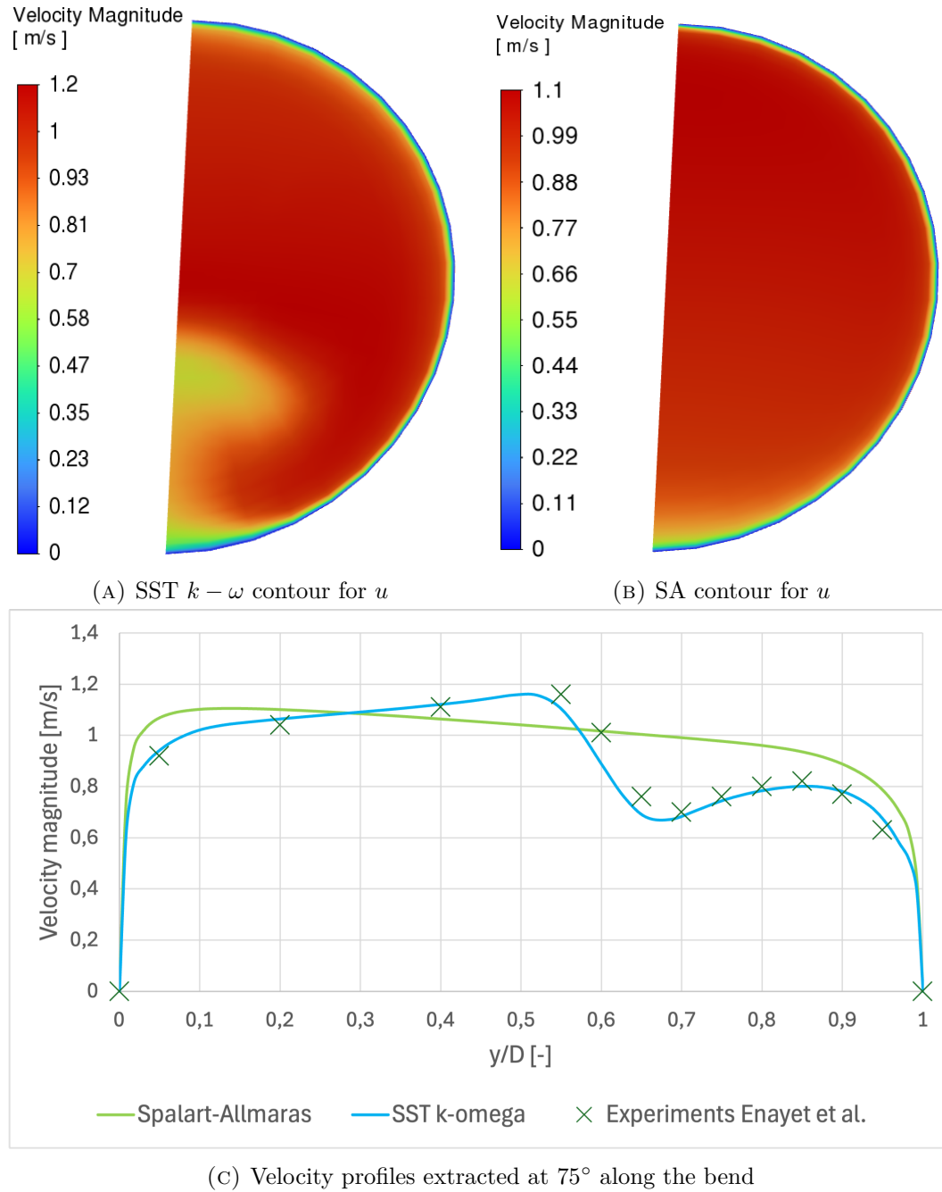
FIGURE 2.10: Flow predictions at the 75^\circ plane along the VMFL030 90^\circ pipe bend. Panels (a) and (b) show velocity contours at the profile plane; panel (c) compares profiles extracted along the pipe diameter from y/D = 0 at the top to y/D = 1 at the bottom. The SA model over-smooths the velocity gradients relative to SST k-\omega and the data of Enayet et al. [22].
