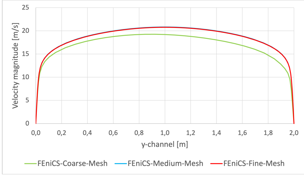
FIGURE A.1: FEniCS wall-normal velocity profiles extracted at x = 0.5L for the Coarse, Medium, and Fine grids in the periodic channel flow benchmark. The overlapping profiles demonstrate asymptotic spatial convergence.
