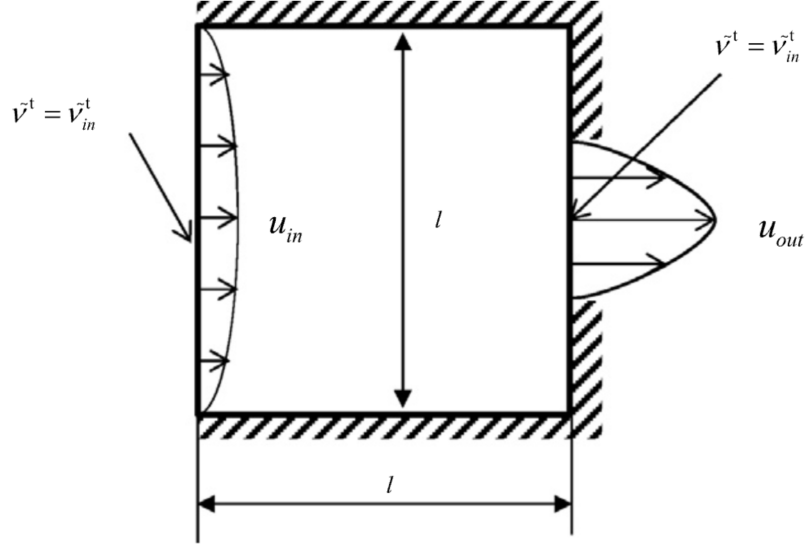
FIGURE 6.11: Geometry and boundary conditions for the velocity-outlet diffuser baseline following Yoon [62]. Both inlet and outlet are prescribed by shifted parabolic velocity profiles.
