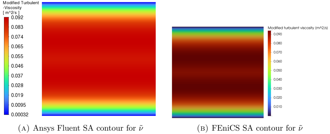
FIGURE 4.3: Comparison of the modified turbulent viscosity \tilde{\nu} , i.e. the Spalart-Allmaras transported working variable, for the 2D channel benchmark. Both solvers drive \tilde{\nu} to zero at the no-slip walls and recover a nearly streamwise-uniform turbulent core.
