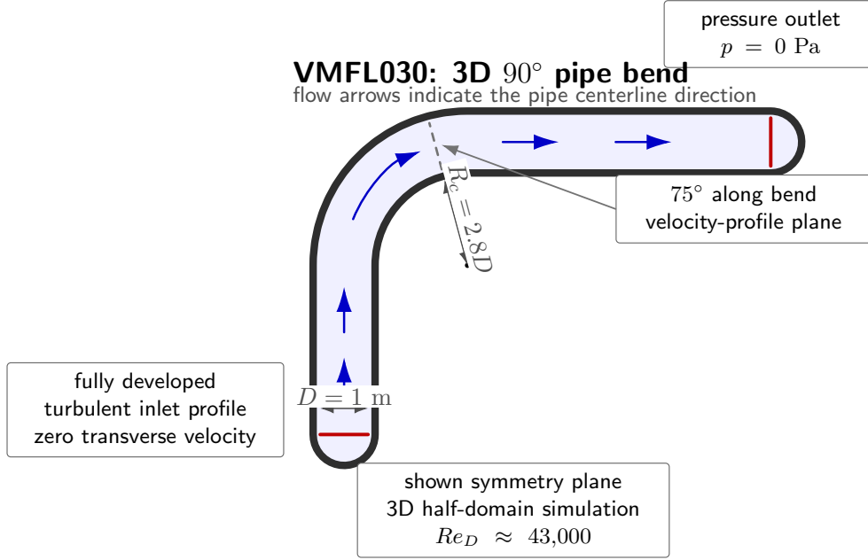
FIGURE 2.9: Geometry and boundary conditions for the VMFL030 3D 90° pipe-bend benchmark adopted from the Ansys Fluid Dynamics Verification Manual [8]. The schematic is not to scale.
