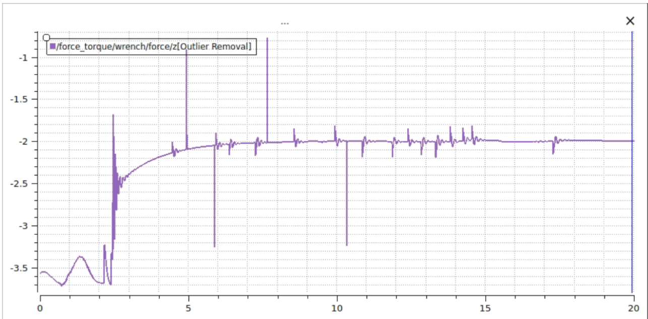
Figure 5: z-axis end-effector force at desire -2 N while UR5e perform drawing task
