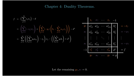
Figure 4.4.2 Proofs of the duality theorems.
