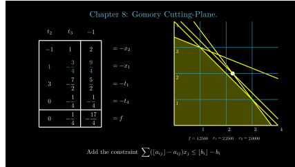
Figure 8.4.2 A demonstration of the Gomory Cutting Plane method.
