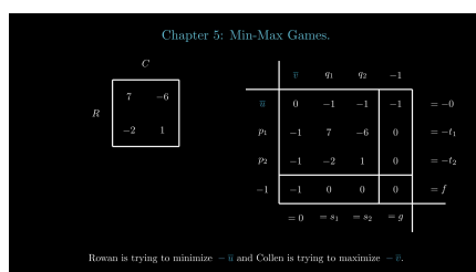
Figure 5.4.1 Zero-Sum Games.
