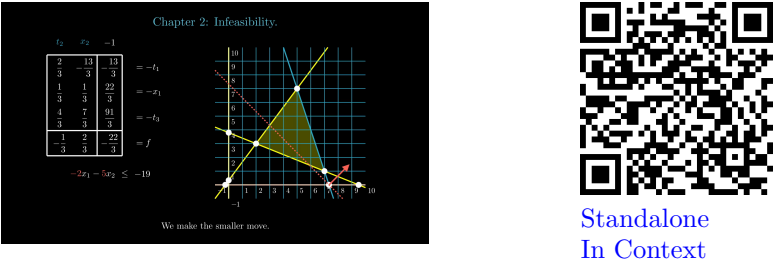
Figure 2.5.4 Infeasible basic solutions and feasible regions.
