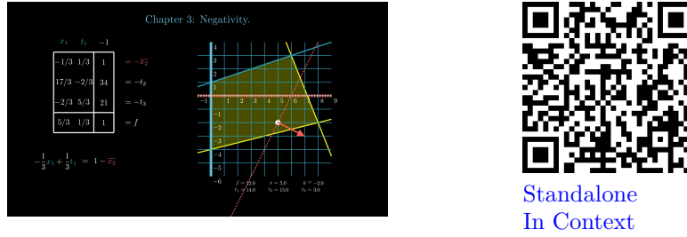
Figure 3.4.1 A summary of unconstrained variables.
