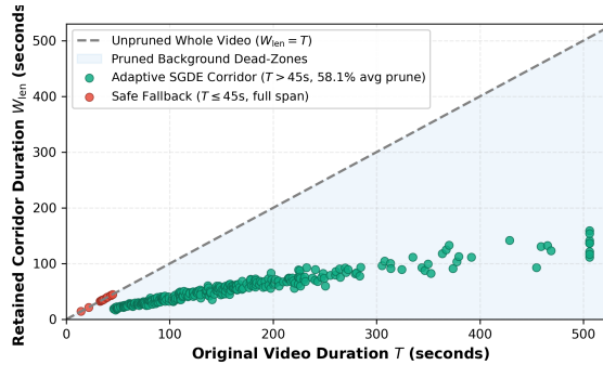
Fig. 3. Original video duration vs. retained candidate corridor duration on OMTG Bench ( N = 320 ). The diagonal dashed line ( W_{\text{en}} = T ) denotes unpruned whole-video baseline. For short videos ( T \leq 45\text{s} ), Adaptive SGDE safely retains the full video span (0% pruned, red points). For longer videos ( T > 45\text{s} ), candidate corridor extraction prunes an average of 58.1% of irrelevant background dead-zones (green points, shaded area), keeping dense decoding tightly focused.
