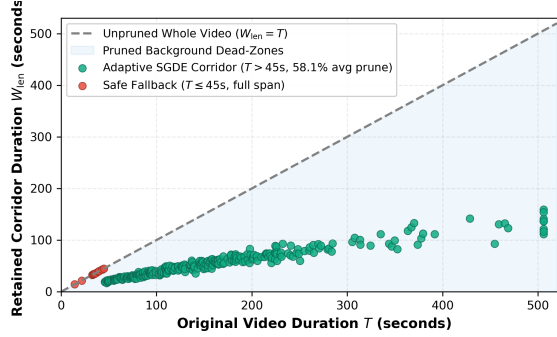
Fig. 2. Original video duration vs. retained candidate window duration on OMTG Bench ( N = 320 ). The diagonal dashed line ( W_{len} = T ) denotes the unpruned baseline. For short videos ( T \leq 45s ), Adaptive SGDE retains the full video span (0% pruned, red points). For longer videos ( T > 45s ), candidate window extraction removes an average of 58.1% of background frames (green points, shaded area).
