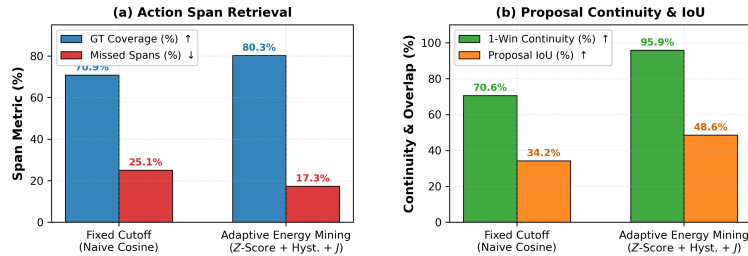
Fig. 3. Evaluation of timeline scoring and candidate extraction methods on OMTG Bench. (a) Action span retrieval: Z-score normalization and energy scoring increase Ground-Truth coverage to 80.3% and cut missed spans by 31.1% relative. (b) Proposal continuity and overlap: achieving 95.9% 1-window continuity and 48.6% proposal IoU.
