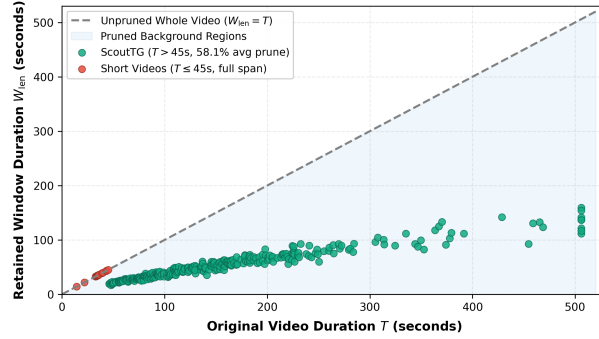
Fig. 2. Original video duration vs. retained candidate window duration on OMTG Bench ( N = 320 ). The diagonal dashed line ( W_{en} = T ) denotes the unpruned baseline. For short videos ( T \leq 45s ), ScoutTG retains the full video span (0% pruned, red points). For longer videos ( T > 45s ), candidate window extraction removes an average of 58.1% of background frames (green points, shaded area).
