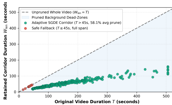
Fig. 3. Original video duration vs. retained candidate corridor duration on OMTG Bench ( N = 320 ). The diagonal dashed line ( W_{\text{len}} = T ) denotes unpruned whole-video baseline. For short videos ( T \leq 45\text{s} ), Adaptive SGDE safely retains the full video span (0% pruned, red points). For longer videos ( T > 45\text{s} ), candidate corridor extraction prunes an average of 58.1% of irrelevant background dead-zones (green points, shaded area), keeping dense decoding tightly focused.
