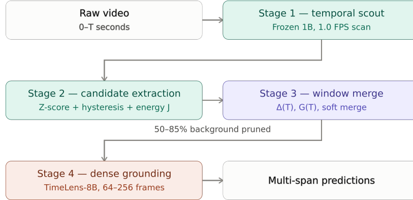
Fig. 1. Overview of Adaptive Scout-Guided Dense Evidence (Adaptive SGDE). Long untrimmed videos are first scanned by a lightweight 1.04B scout at 1.0 FPS. Local Z-score normalization and thresholding extract candidate action proposals, which are grouped by duration-adaptive windowing and continuity merging. The focused candidate window is decoded with dense frames by a frozen 8B Vision-Language model using schema-delimited JSON syntax, removing background frames while preserving event cardinality.
