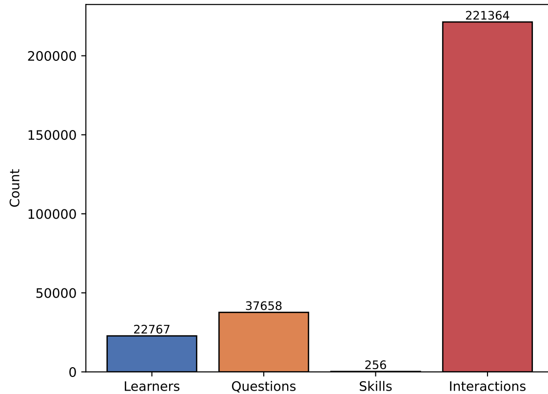
Dataset Statistics
