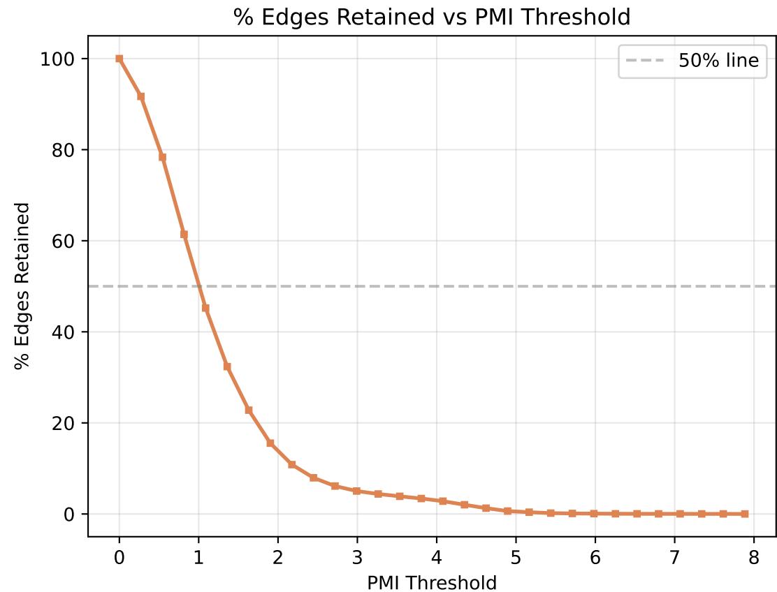
Fig 5: E_co Threshold Sensitivity — assist2012 fold 0
