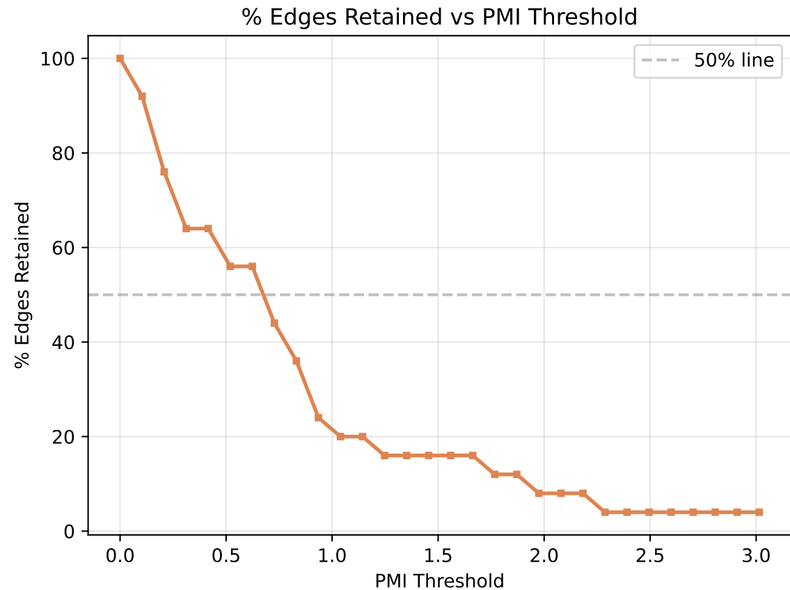
Fig 5: E_co Threshold Sensitivity — junyi fold 0
