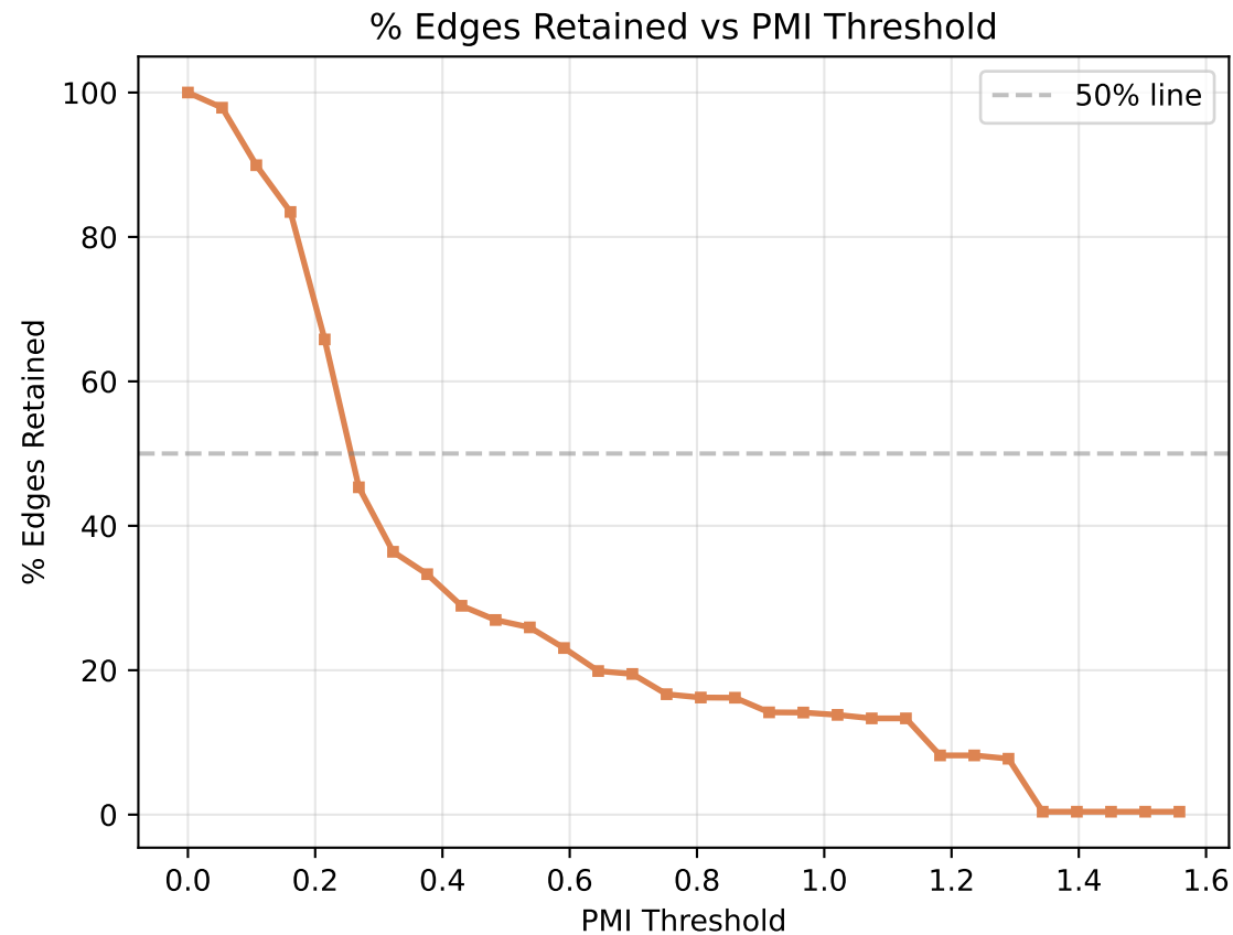
Fig 5: E_co Threshold Sensitivity — kdd2010 fold 0
