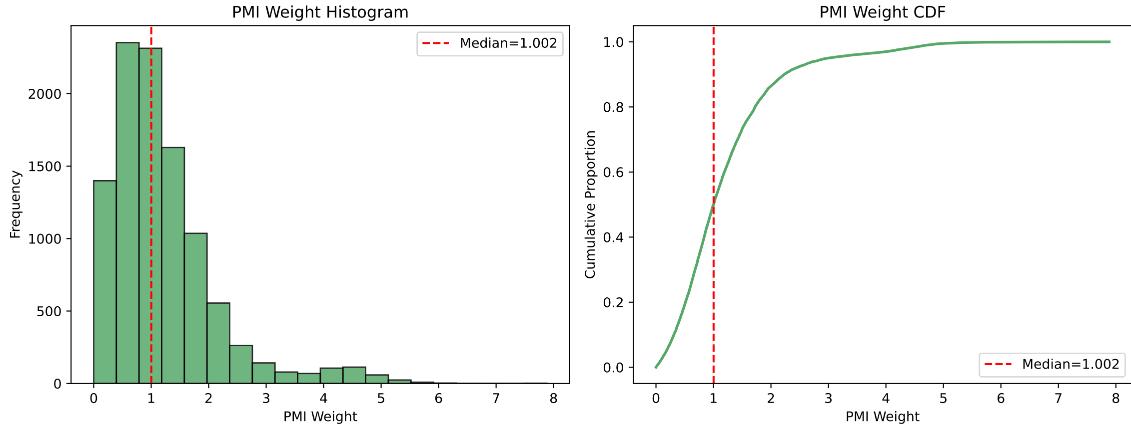
Fig 2: E_co Weight Distribution — assist2012 fold 0
