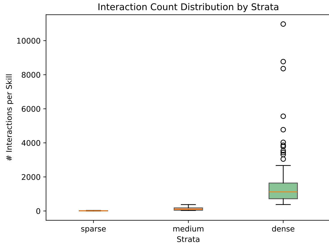
Fig 3: Sparse-Skill Strata — assist2012 fold 0
