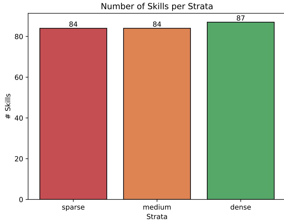
Fig 3: Sparse-Skill Strata — assist2012 fold 0
