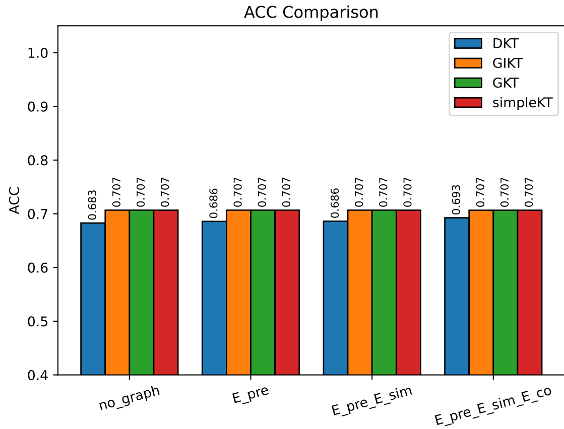
Fig 4: Relation Ablation — assist2012 fold 0
