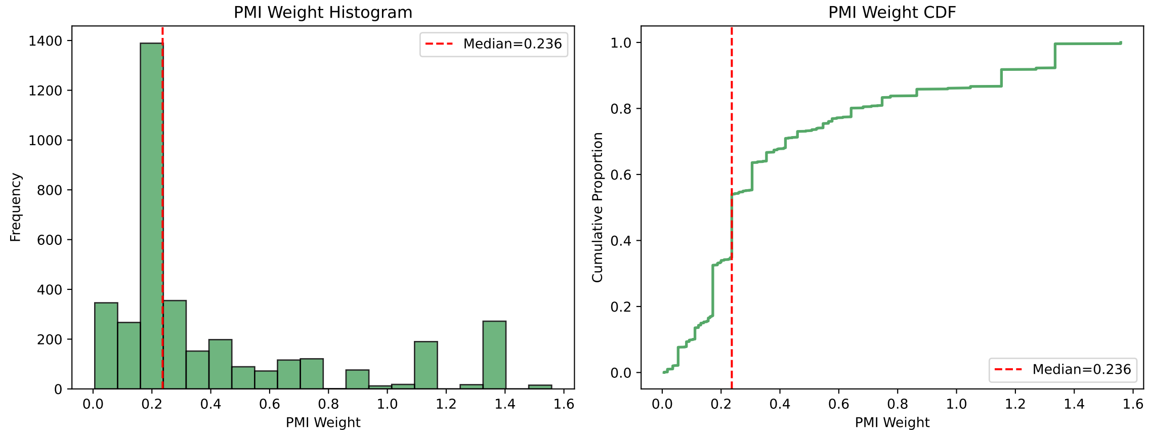
Fig 2: E_co Weight Distribution — kdd2010 fold 0
