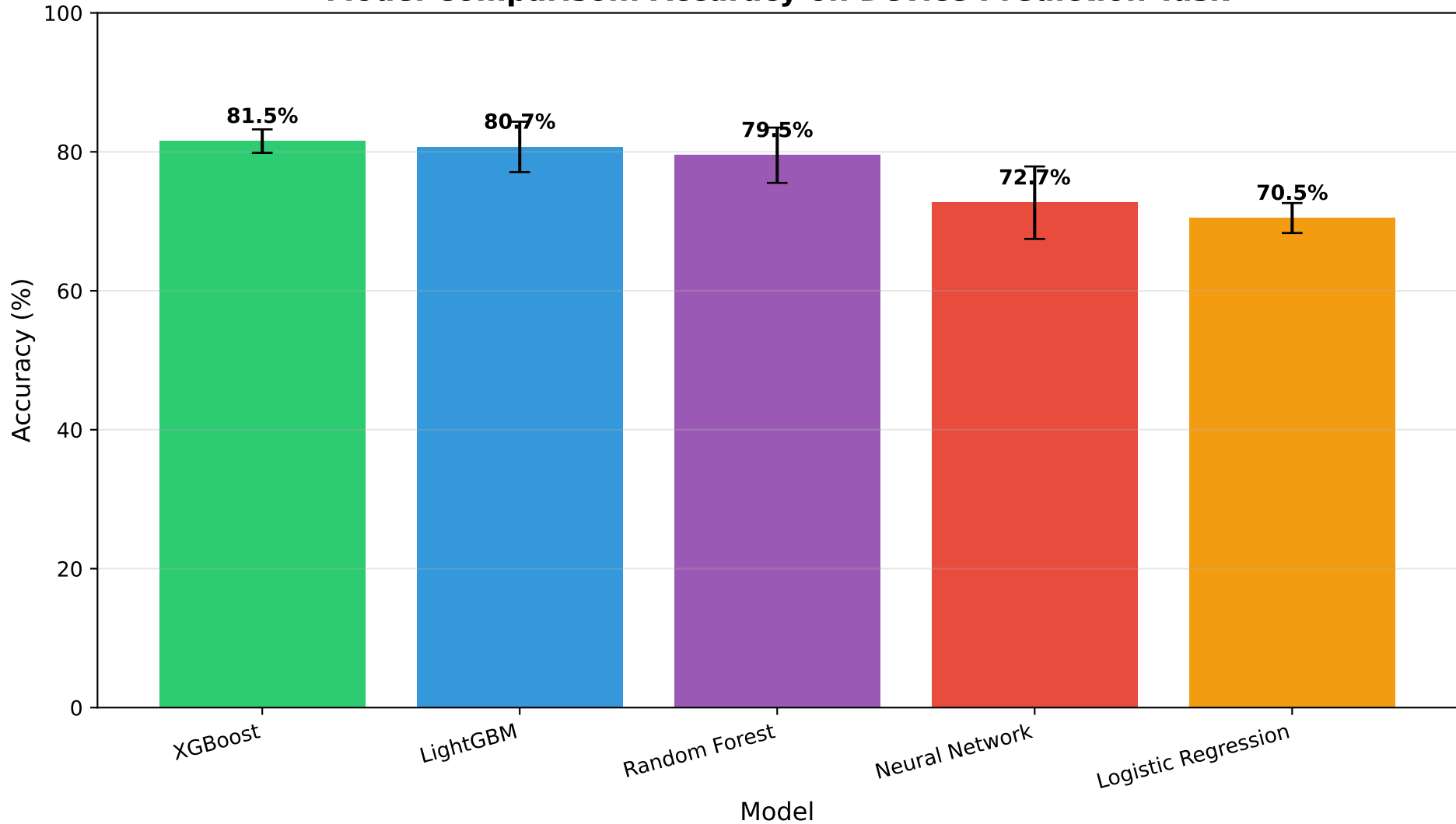
Model Comparison: Accuracy on Device Prediction Task
