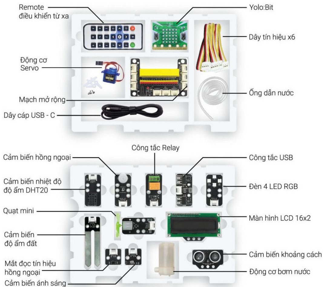
Figure 2.2: OhStem AIoT Kit and its main hardware modules.
