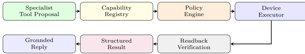
Figure 3.4: Safe tool execution path for effectful device-control requests.
