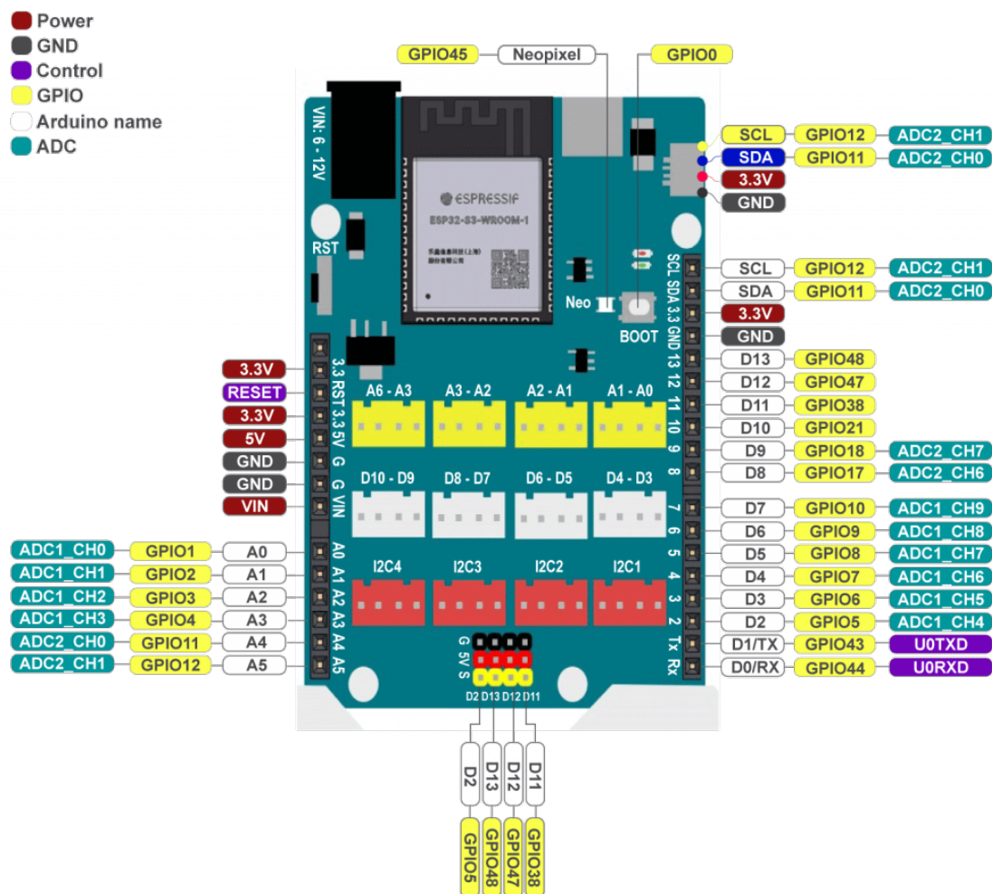
Figure 2.1: ESP32-S3-N16R8 based Ohstem Yolo UNO development board and pinout.
