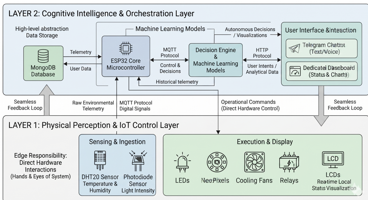
Figure 1.1: System Architecture of H.E.R.A
