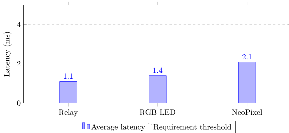
Figure 7.1: Average RPC command execution latency compared with the required threshold
