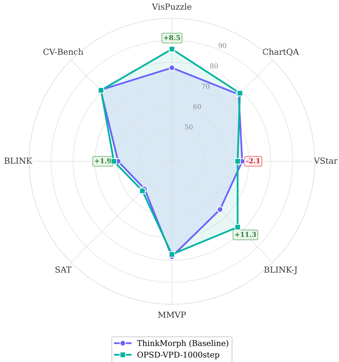
(a) Baseline vs. Best Checkpoint
