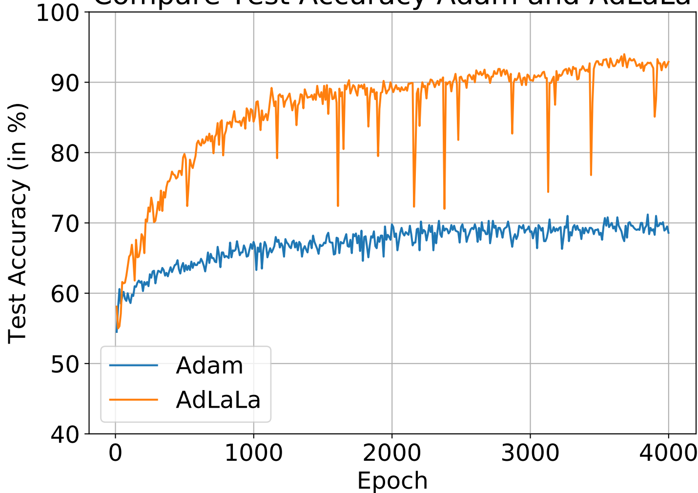
Compare Test Accuracy Adam and AdLaLa
