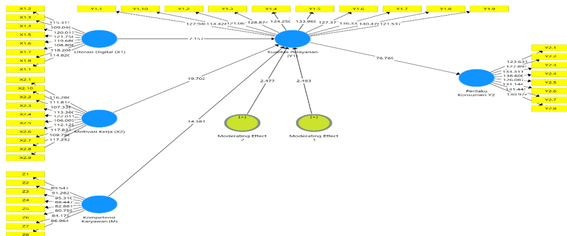
Gambar 2. Outer Model
