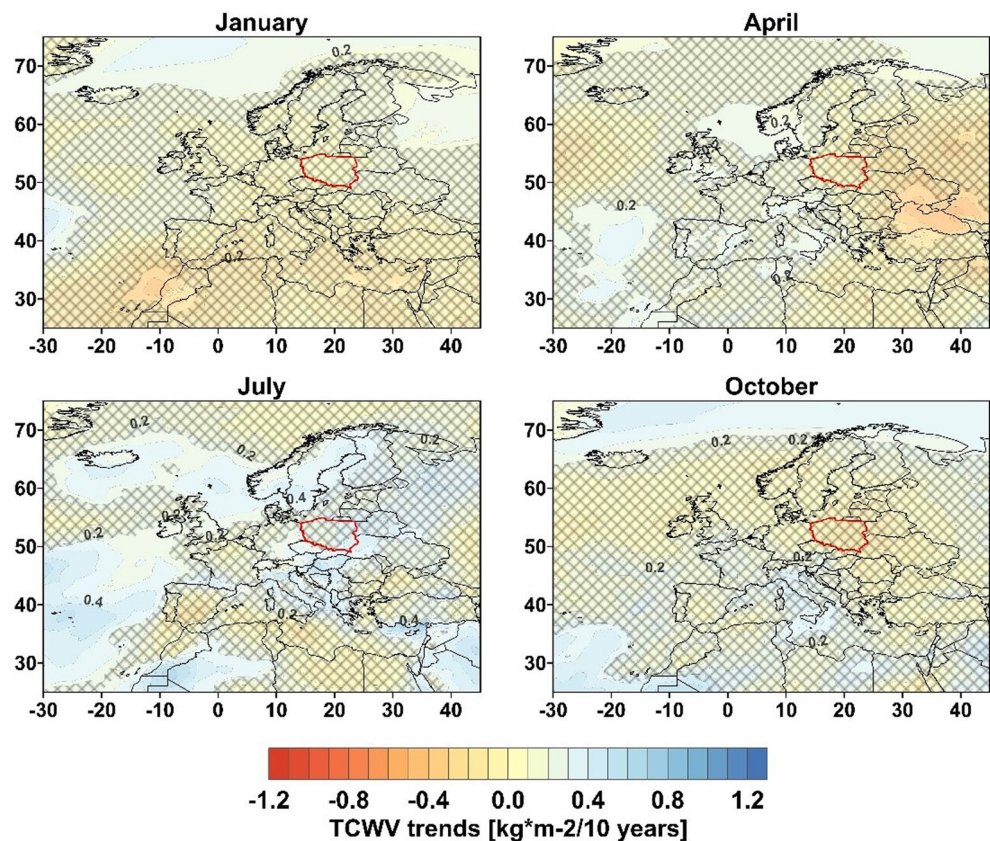
Fig. 7 Trends of monthly total column water vapour over Europe in January, April, July and October in 1966–2020; shaded areas are statistically insignificant
