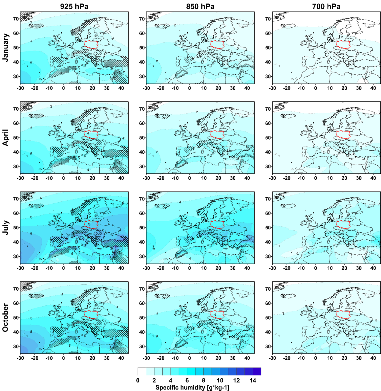
Fig. 4 Distribution of the monthly mean of specific humidity over Europe in January, April, July and October at the pressure levels of 925, 850 and 700 hPa; the shaded areas were excluded due to the lowest altitude of the pressure levels below the surface level
