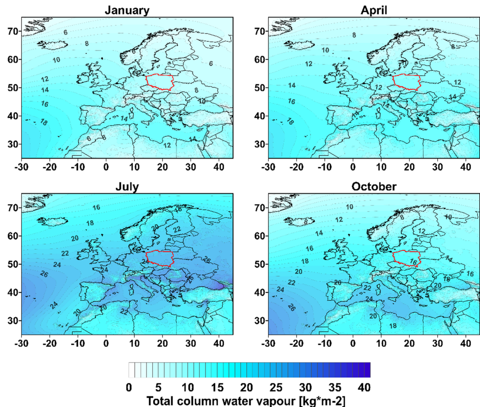
Fig. 2 Monthly mean of total column water vapour over Europe in January, April, July and October in 1966–2020
