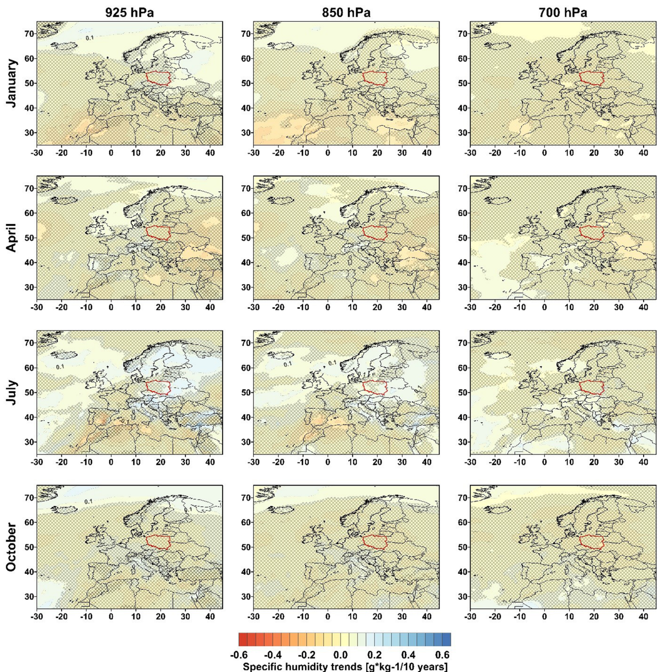
Fig. 8 Trends of monthly specific humidity in January, April, July and October at the pressure levels of 925, 850 and 700 hPa over Europe in 1966–2020; shaded areas are statistically insignificant
