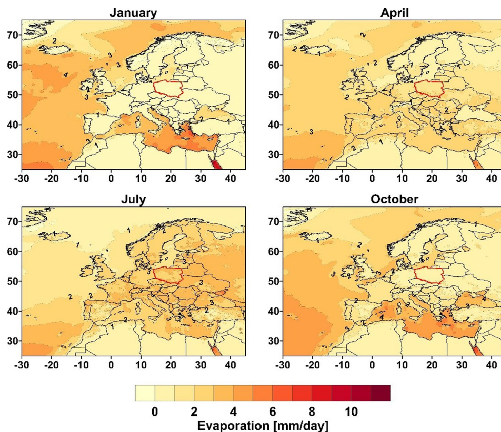
Fig. 3 Monthly mean of actual evaporation (mm/day) over Europe in January, April, July and October in 1966–2020
