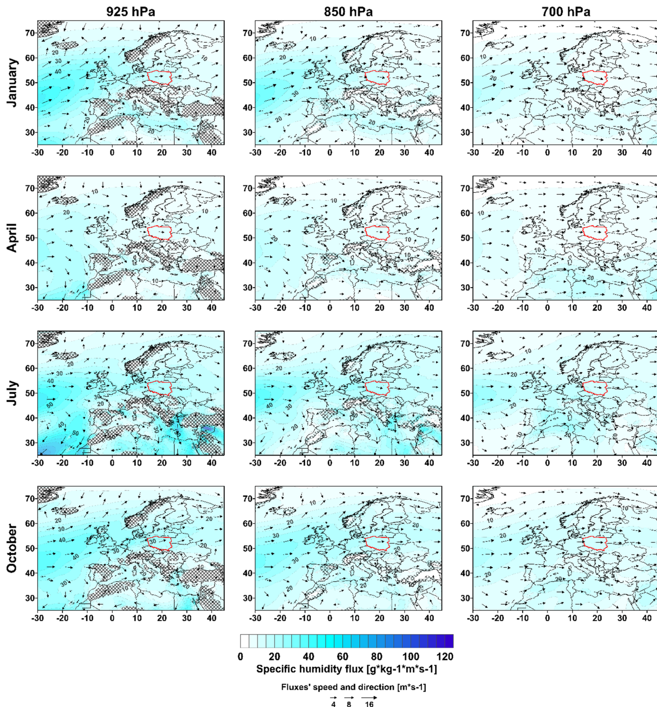
Fig. 5 Monthly mean of specific humidity fluxes in January, April, July and October and characteristics of horizontal advection of water vapour over Europe at the pressure levels of 925, 850 and 700 hPa; the
