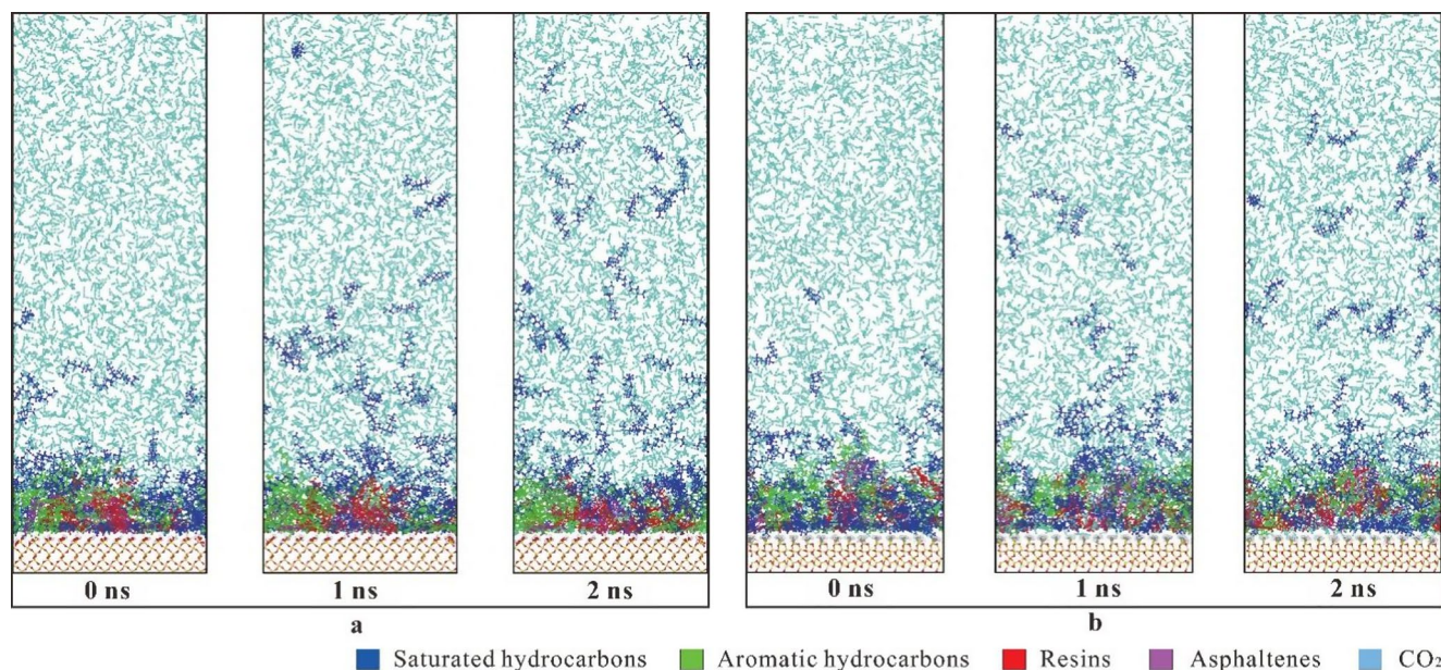
Fig. 3 (a) CO_2 extraction of hydroxylated SiO_2 surfaces crude oil; (b) CO_2 extraction of methylated SiO_2 surfaces crude oil [40]
