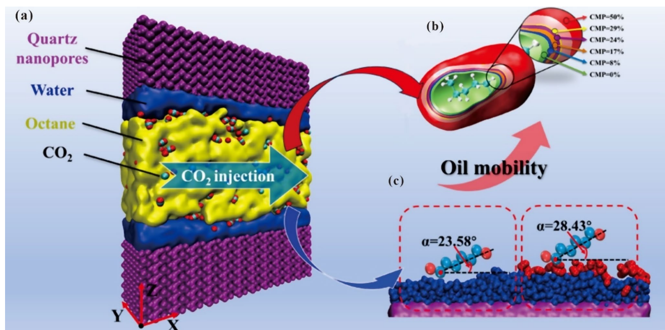
Fig. 2 Molecular Distribution and Velocity Profiles of nC8, Water, and CO 2 in Quartz Nanopores, (a) Mass Density Distributions of nC8, Water, and CO 2 in Quartz Nanopores, (b) Spatial distribution functions
