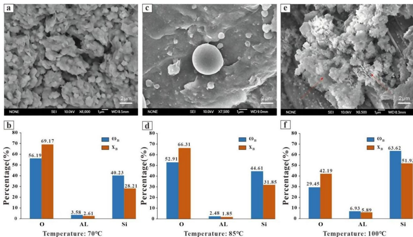
Fig. 14 The formation process of new minerals; (a) Acicular minerals formed after reaction at 70°C; (b) The mass fraction and atomic fraction of the acicular mineral at 70°C; (c) Spherical minerals formed after reaction at 85°C; (d) The mass fraction and atomic fraction of the spherical mineral at 85°C; (e) Acicular and floral minerals formed
