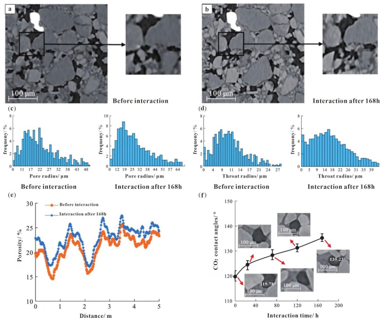
Fig. 12 Microscopic evolution of sandstone reservoir properties induced by CO 2 -brine-rock interactions during CO 2 flooding and storage. (a) Initial microscopic morphology of sandstone pore structure before interaction; (b) Pore structure morphology after 168 h of CO 2 -brine-rock interaction; (c) Changes in pore radius distribution before
