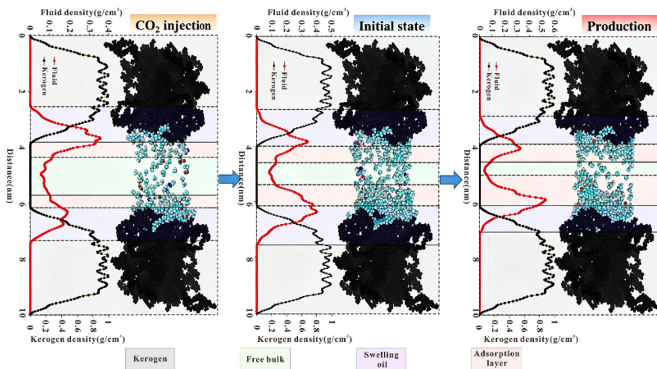
Fig. 8 The adsorption characteristics of shale oil in kerogen at three production stages (2 nm). Components color scheme: black, kerogen I-A. Elements color scheme: cyan, C; blue, N; red, O; white, H; purple,
