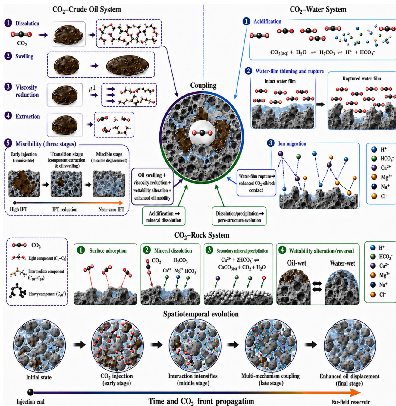
Fig. 1 Schematic diagram of multiphase coupling microscopic interactions and spatiotemporal evolution of CO 2 -oil-water-rock system
