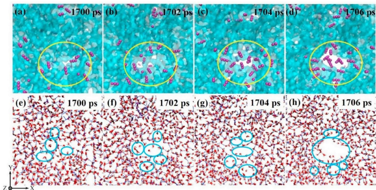
Fig. 9 Details (top View) of carbon dioxide diffusing into the water film at (a) t = 1700 ps, (b) t = 1702 ps, (c) t = 1704 ps, and (d) t = 1706 ps, and snapshots (top View) of hydrogen bonds in the water film at (e) t = 1700 ps, (f) t = 1702 ps, (g) t = 1704 ps and (h) t = 1706 ps. The blue circles highlight where the hydrogen bonds have been broken
