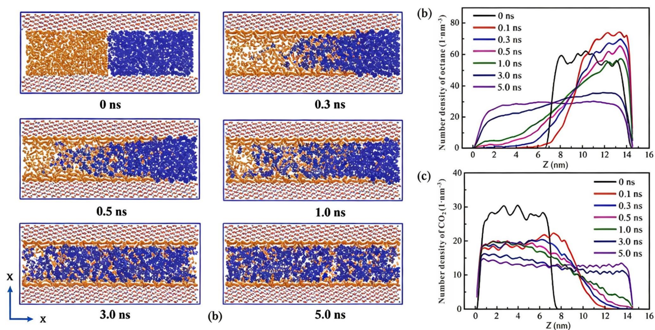
Fig. 4 (a) The snapshot of the miscible process of CO 2 and octane, the number density profiles along the Z direction. (b) Octane, (c) CO 2 [43]
