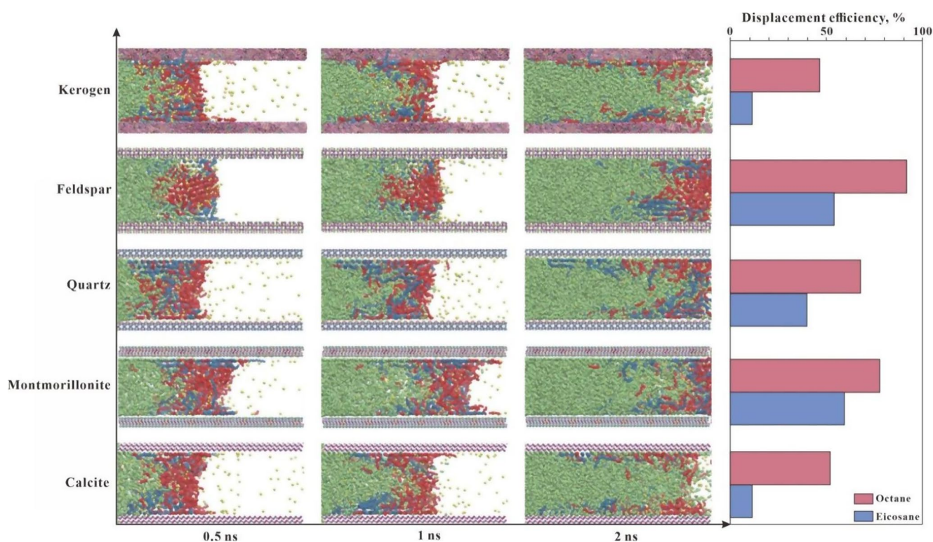
Fig. 6 Molecular dynamics configurations and displacement efficiency of octane and eicosane during CO 2 flooding in different shale nanopores at 0.5 ns, 1 ns, and 2 ns. The color markings are CO 2 (green), methane (yellow), octane (red), and eicosane (dark blue) [58]
