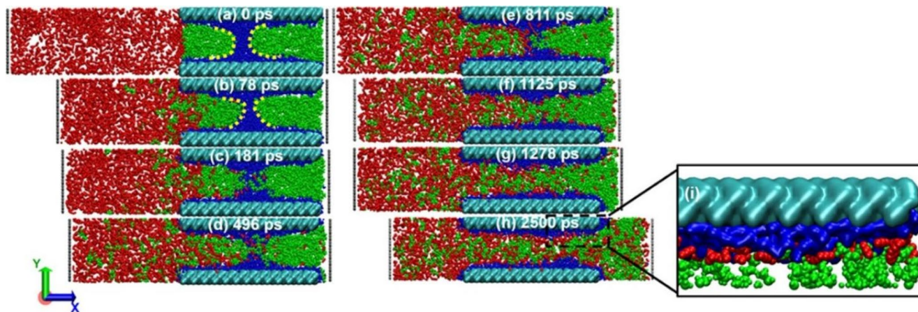
Fig. 10 Snapshot of \text{CO}_2 breaking through the water bridge at typical moments: (a) 0 ps, (b) 78 ps, (c) 181 ps, (d) 496 ps, (e) 811 ps, (f) 1125 ps, (g) 1278 ps, and (h) 2500 ps. The configuration of water/octane/ \text{CO}_2 molecules near the upper surface at 2500 ps is enlarged in figure
