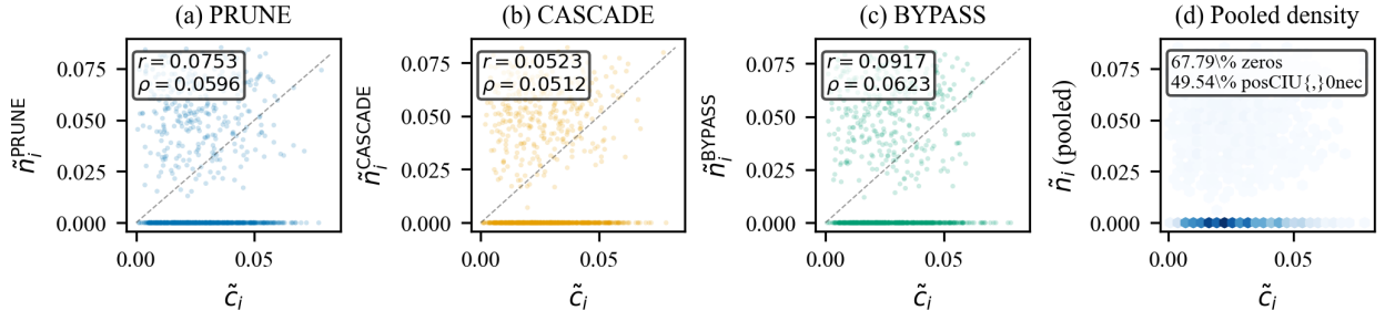
Figure 2: Structural diagnostic motivating calibration. Local utility and graph-level necessity are not interchangeable: many locally useful steps have low measured structural necessity, while some structurally exposed steps do not receive strong local utility signals. SC-FMA uses this mismatch as the reason for calibration.
