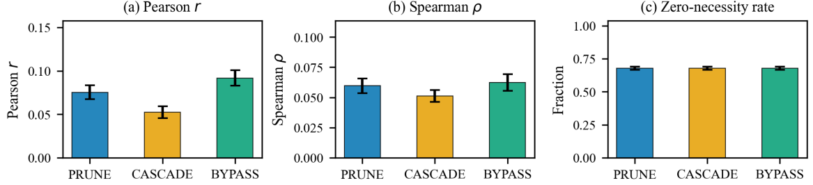
Fig. 3 Structural perturbation summary by mode. The three perturbation modes (PRUNE, CASCADE, BYPASS) are reported with Pearson correlation, Spearman annotation-order consistency, and zero-necessity fraction. Error bars indicate 95% bootstrap confidence intervals. The consistency across modes indicates that weak local-utility–necessity alignment persists across perturbation strategies.
