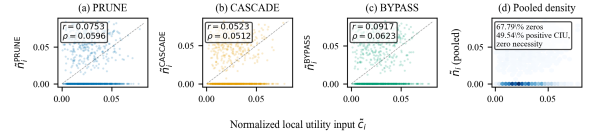
Fig. 2 Structural mismatch motivating calibration. Local utility and graph-level necessity diverge: many locally useful steps have low measured structural necessity, while some structurally exposed steps receive limited local utility support. The shared x -axis \tilde{c}_i denotes the normalized local utility field for step i . SC-FMA uses this mismatch as the reason for calibration.
