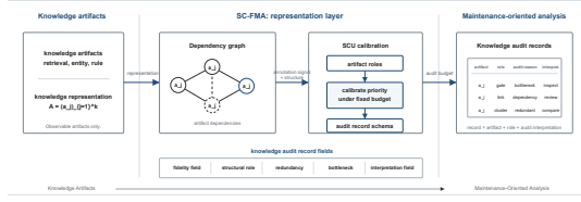
Fig. 1 Knowledge engineering workflow for dependency-aware audit records. The figure should be read as a transformation from Knowledge Artifact \rightarrow Representation \rightarrow Graph Structure \rightarrow SCU \rightarrow Audit Record \rightarrow Knowledge Curation. Raw reasoning traces, graph nodes, and process annotations are first organized as auditable knowledge artifacts, then represented through dependency-aware graph structure. SCU constructs structured audit records by preserving annotation or utility fidelity while adding structural dependency, redundancy, bottleneck, audit-reason, and interpretation fields. The resulting records support fixed-budget audit representation and analysis; the audit-priority field is only a downstream use of the audit representation.
