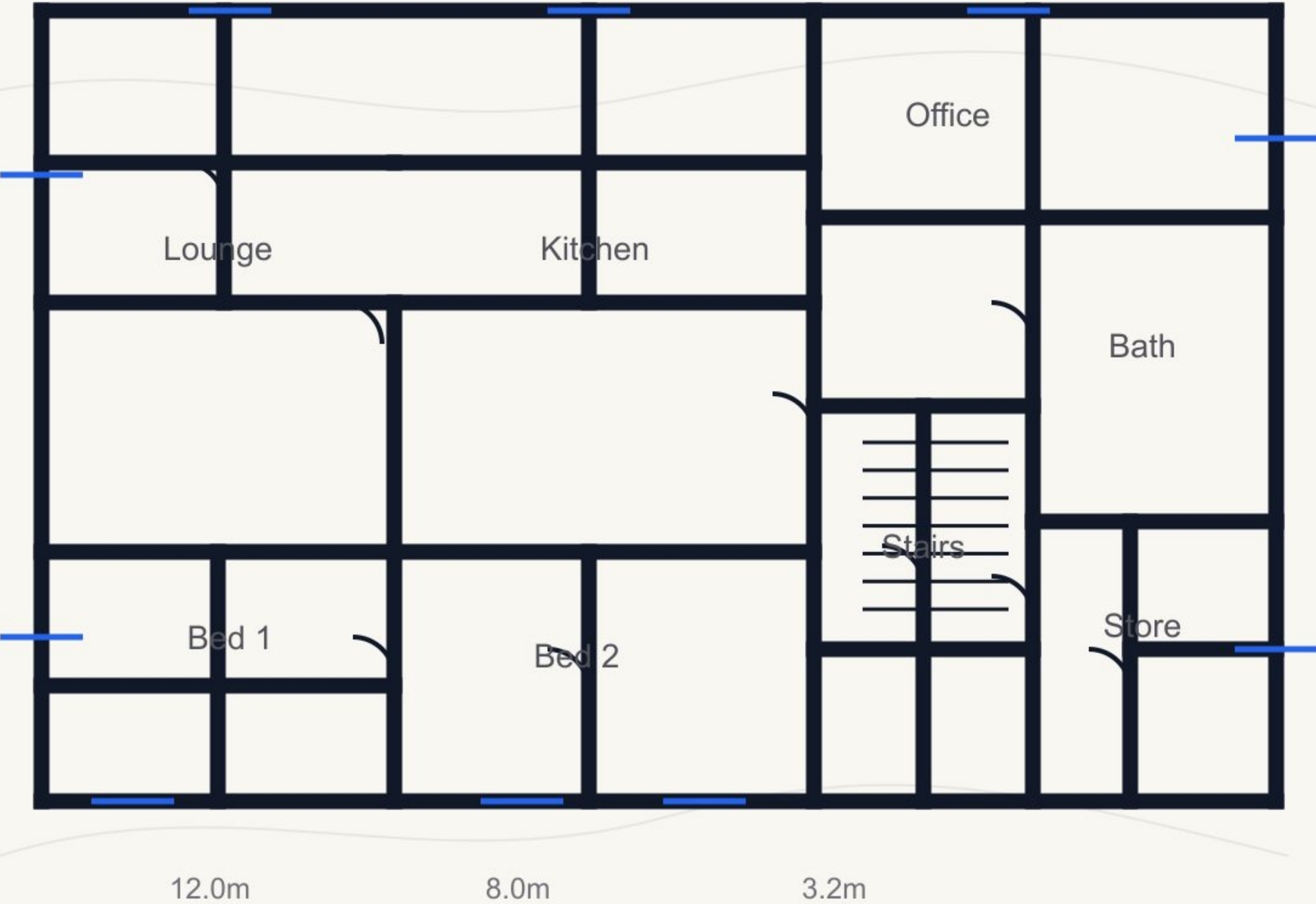
Dimensioned scanned plan with stairs
