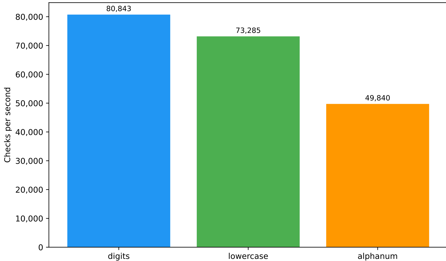
Password Check Speed by Charset
