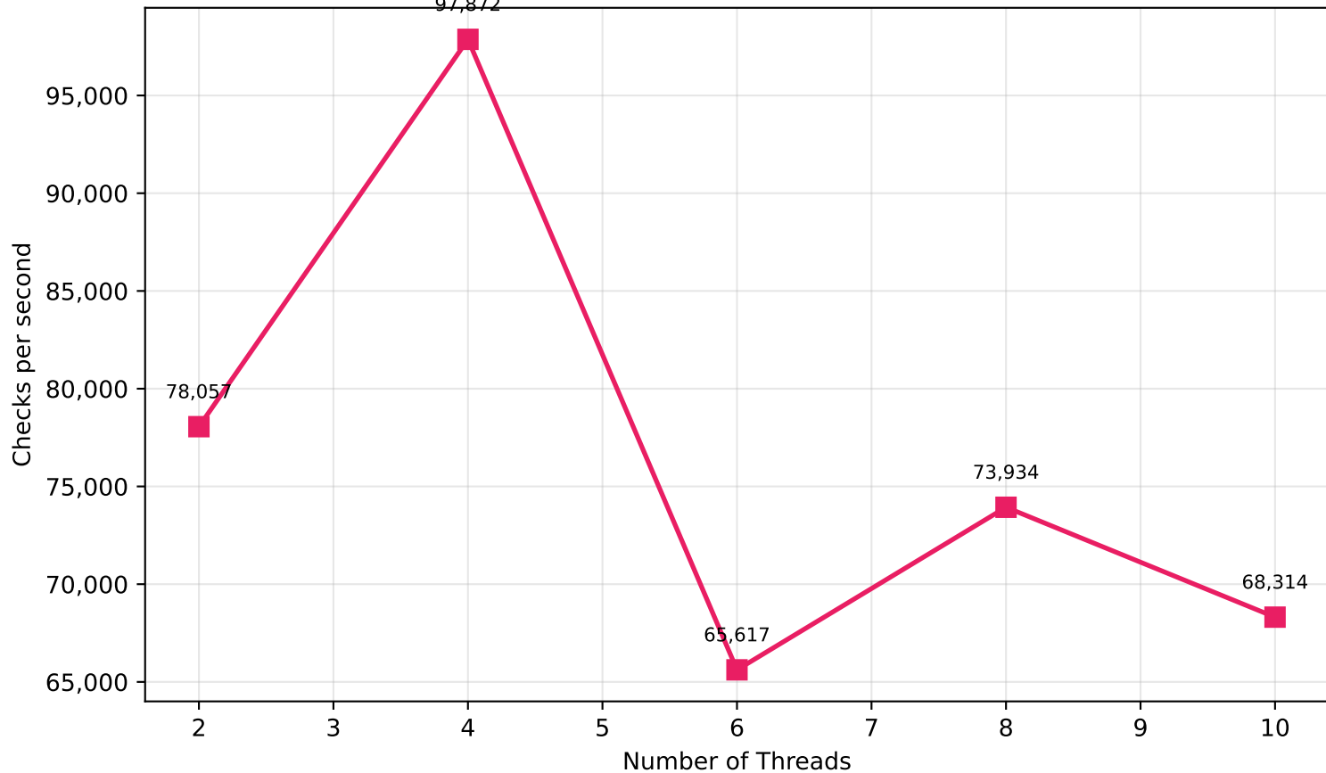
Performance Scaling: Checks/sec vs Threads
