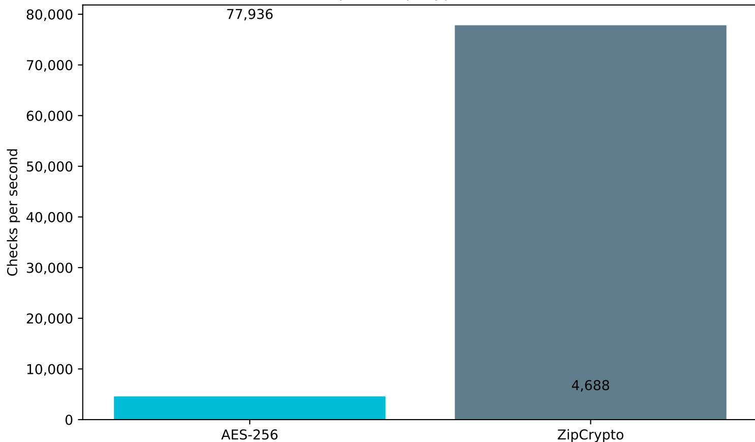
Check Speed: ZipCrypto vs AES-256
