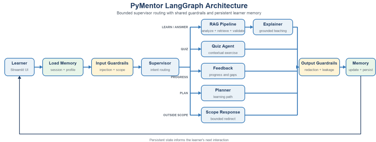
Figure 1. PyMentor architecture: bounded LangGraph routing with shared guardrails and persistent learner memory.
