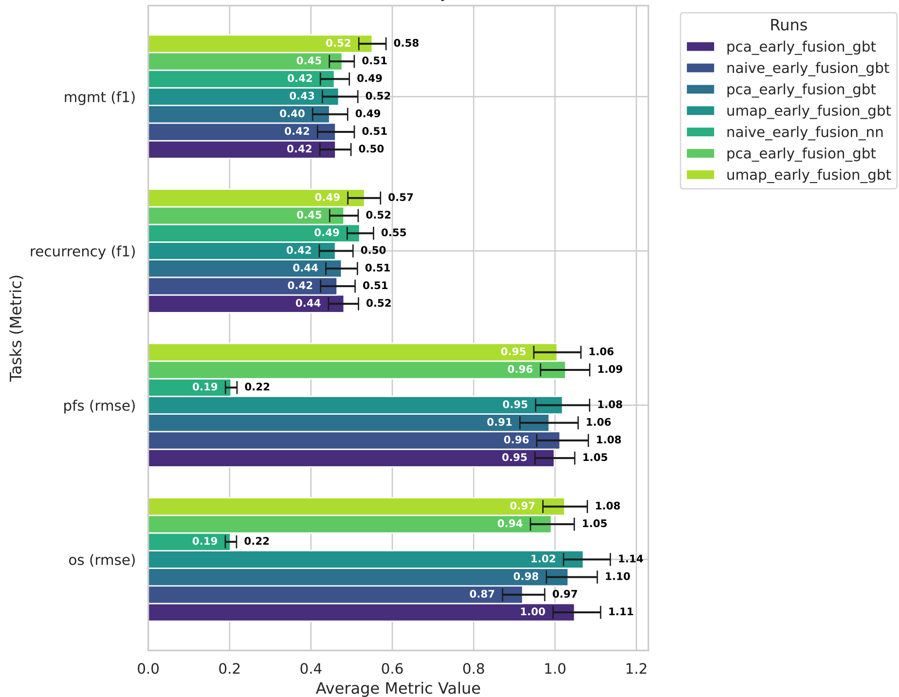
Cross-Validation Results by Task and Run
