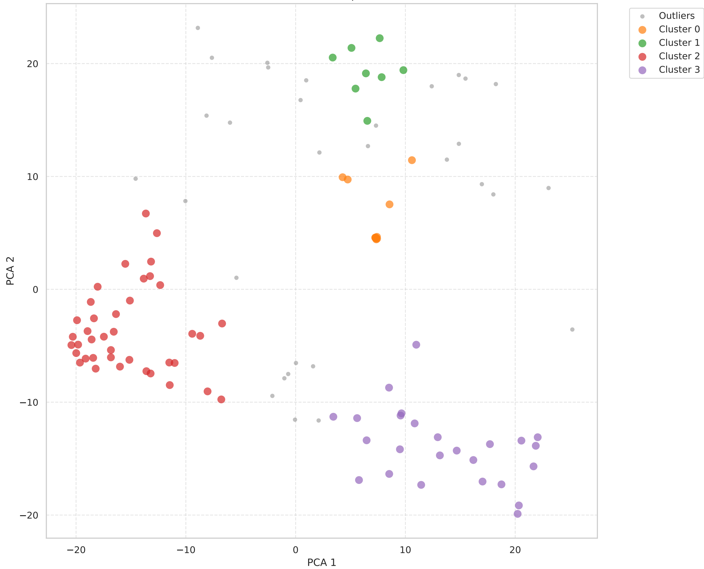
PCA of 114 samples
