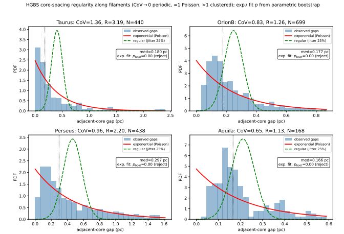
Figure 7. Adjacent-core gap distributions along the skeletons of the four primary regions (histograms), with exponential/Poisson (solid) and regular/periodic (dashed) reference curves; each panel gives the coefficient of variation CoV, the 1-D Clark–Evans ratio R , and the exponential goodness-of-fit p -value calibrated by parametric bootstrap ( p_{\text{boot}} ; the null distribution of the KS statistic is built by resampling from the fitted exponential, removing the estimated-parameter bias of the standard test). The result is two-sided: the regular/periodic model is rejected overwhelmingly ( p_{\text{boot}} < 10^{-3} , the parametric-bootstrap floor, 1/N_{\text{boot}} with N_{\text{boot}} = 10^3 ) in every region, and the pure-exponential (Poisson) model is also rejected ( p_{\text{boot}} \leq 0.002 in all four), so the cores are neither periodic nor pure-Poisson — consistent with a clustered process bearing a beam-scale exclusion (the deficit of small gaps, R > 1 ; largely instrumental).
