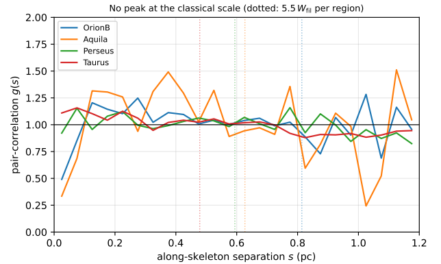
Figure 6. Along-skeleton pair-correlation function g(s) for the four primary clouds (uniform-random expectation on the matched components divided out; g = 1 is no correlation). Dotted vertical lines mark the classical scale 5.5W_{\text{fil}} per region. No cloud shows a peak at the classical scale ( g \approx 1 there, slightly below unity in Orion B and Aquila); the only departures are a mild small-separation excess (Taurus) and weak region-envelope features near 1\text{ pc} . The classical periodic comb is therefore absent, consistent with a non-periodic, intermittent distribution bearing a small-scale exclusion (Section 2.9).
