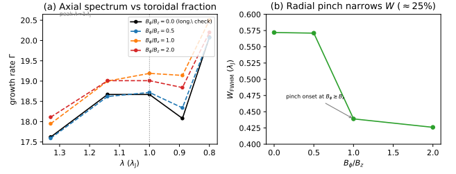
Figure 11. Divergence-free helical-field scan ( B_\phi/B_z = 0 –2, 512 \times 128^2 ; Section 4.3). (a) The axial growth-rate spectrum \Gamma(\lambda) in the physical band is invariant to the toroidal fraction ( < 6\% , fit noise), with the plateau peak fixed at \lambda \approx 1 \lambda_J ; B_\phi/B_z = 0 (black) reproduces the pure-longitudinal spectrum, a code check. No excess growth appears at shorter \lambda for any winding. (b) The one systematic effect is a radial pinch : the formation FWHM narrows by \approx 25\% , with onset at B_\phi \gtrsim B_z . The seeded helical field therefore raises \lambda/W by shrinking W , not by shortening \lambda ; the force-balanced Fiege & Pudritz (2000) pinch mode is not tested here.
