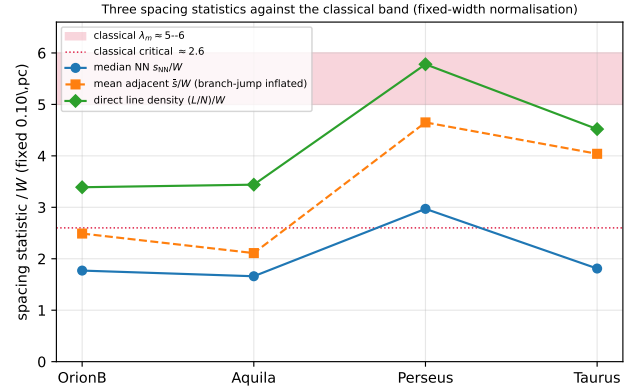
Figure 5. Three spacing statistics per cloud (single re-implementation, all normalised by the fixed 0.10\text{ pc} width so they are directly comparable), against the classical band ( 5\text{--}6 , red; critical \approx 2.6 , dotted). The median along-skeleton ACS spacing (blue, \approx 1.7\text{--}3.0 ) is sub-classical everywhere; the direct line density (L/N)/W (green, \approx 3.4\text{--}5.8 ) is classical in Perseus, near-classical in Taurus, and sub-classical in Orion B and Aquila; the mean adjacent spacing (orange) lies between but is inflated by arc-length branch-jumps. The factor- \approx 2 gap between the blue and green points reflects the generic mean/median skew plus dilution by core-poor filament (a coverage effect), not small-scale clustering (Section 2.8): short adjacent spacing within core-bearing stretches, diluted by extensive core-free filament.
