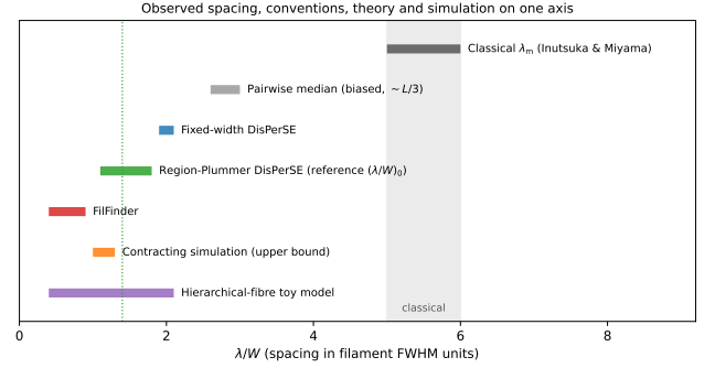
Figure 8. The full methodological envelope of \lambda/W on a single axis, showing that several distinct physical interpretations occupy the allowed observational region while all lie well below the classical value. Marked, from top: the classical band (5–6; Inutsuka & Miyama 1992; Fischera & Martin 2012); the biased pairwise median ( \approx L/3 ); fixed-width DisPerSE (1.9–2.1); region-Plummer DisPerSE (our reference ACS-spacing ratio (s_{\text{ACS,med}}/W)_0 \approx 1.4 ); FilFinder (0.4–0.8, Table 4); the contracting-simulation upper bound (1.0–1.3); and the hierarchical-fibre toy-model range. Because the observational conventions, the simulated upper bound and the fibre toy model all overlap well below the classical band, the sub-classical sign is robust while its magnitude is convention-dominated (Section 2.13); the comparison with simulation (Section 5) should be read against this envelope, not against a single number. (Point ranges are descriptive, not confidence intervals; Section 2.10.)
