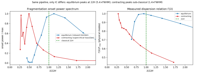
Figure 14. Equilibrium-recovery control (the primary validation that the sub-classical spectrum is not generated by the wavelength-extraction pipeline and is associated with the non-equilibrium initial state). The identical growth-rate measurement pipeline is applied to a relaxed, force-balanced pressure-confined Ostriker equilibrium (blue; prepared by explicit drag relaxation, then evolved drag-free) and to a dynamically contracting supercritical filament (orange); the two differ in their prepared initial state, not in the measurement, isolating the effect of starting from equilibrium versus contraction. Left : onset fragmentation power spectrum; the equilibrium peaks at the classical \lambda_m \approx 22H ( \approx 5.4 W_{\text{FWHM}} ) while the contracting filament peaks sub-classically ( \approx 1.4 W_{\text{FWHM}} , upper limit). Right : the dispersion relation \Gamma(\lambda) versus \lambda/22H ; the equilibrium shows the classical peak-and-decline with its maximum at 22H , whereas the contracting filament's \Gamma rises monotonically. The pipeline thus recovers the classical wavelength when the physics is classical.
