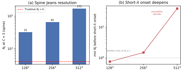
Figure 10. Ideal perpendicular-field refinement ladder ( 128^3 – 512^3 ; Section 4.3). (a) Cells per local Jeans length N_J at the beading-relevant spine contrast C \approx 3 : the collapsing spine is resolved far above the Truelove threshold ( N_J = 4 , dashed) at every resolution. (b) The spurious short- \lambda axial “beading” emerges only once the spine drops below N_J \approx 1 , and refinement pushes that onset to ever-deeper collapse (at 512^3 the filament stays monolithic to N_J \approx 40 at C \approx 30 ) — the short- \lambda onset deepening with resolution being the textbook Truelove under-resolution artefact signature, not a physical fragmentation mode.
