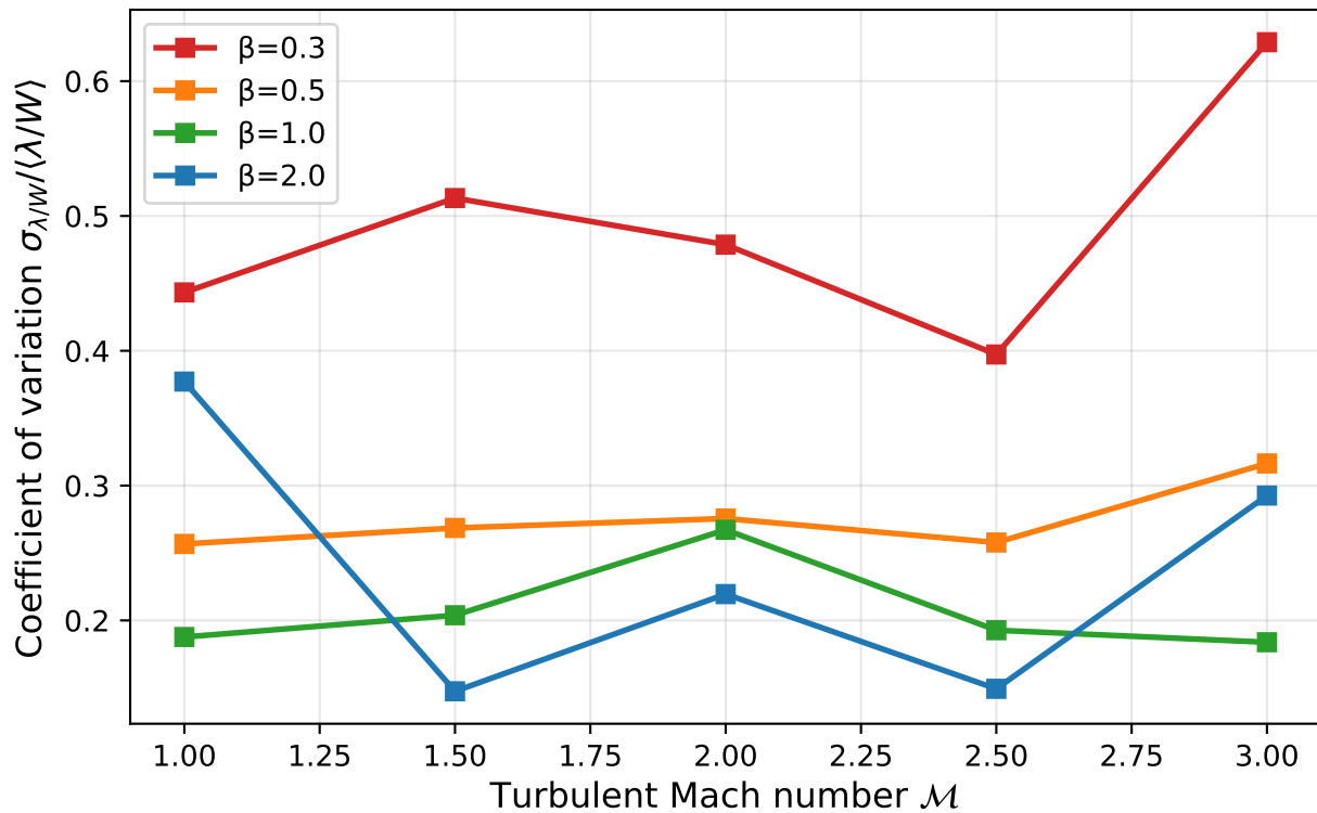
(b) Stochastic scatter vs \mathcal{M} (flat \rightarrow turbulence doesn't set the scale)
