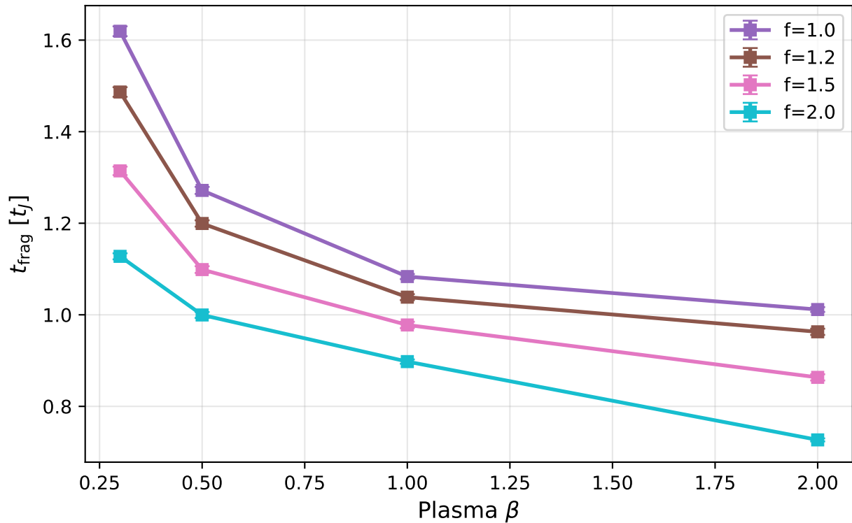
(b) Fragmentation time vs \beta (stronger field delays collapse)
