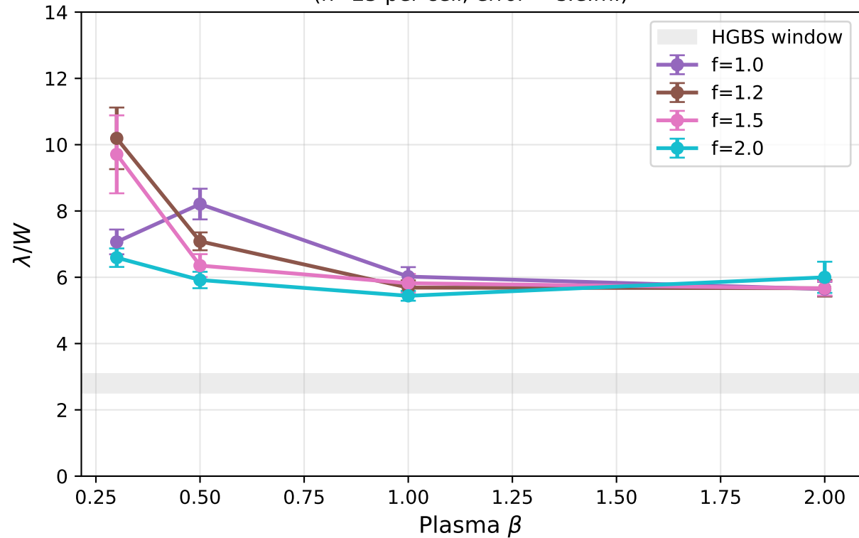
(a) \lambda/W vs \beta — controlling variable ( n=25 per cell, error = s.e.m.)
