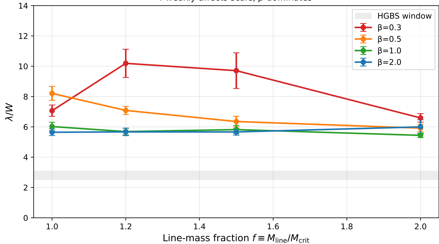
\lambda/W vs line-mass fraction f (longitudinal field, all Mach averaged) f weakly affects scale; \beta dominates
