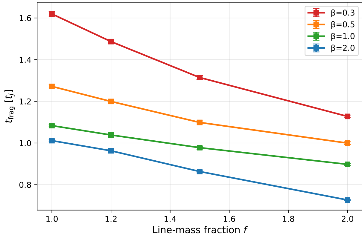
(b) t_{\text{frag}} vs f — clear trend (higher f = faster collapse)
