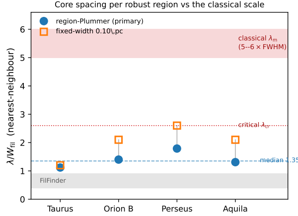
Figure 4. Adjacent-core (ACS) core spacing per primary region ( s_{\text{ACS,med}}/W_{\text{fil}} ; Section 2.10), in the two DisPerSE width conventions: directly-measured region-Plummer widths (blue circles, preferred; per-region raw 1.1, 1.4, 1.8, 1.3, dashed line at the median, which we quote as 1.4; the rounded median of these four values, whose exact median is 1.35) and the fixed 0.10 pc width (orange squares; 1.2, 2.1, 2.6, 2.1), both shown raw (before the injection–recovery correction; Section 2.7). The red band is the classical fastest-growing wavelength \lambda_m \approx 5\text{--}6 \times \text{FWHM} (Fischera & Martin 2012; = 4 \times the flat diameter, Inutsuka & Miyama 1992) and the dotted line the classical critical wavelength \lambda_{\text{cr}} \approx 2.6 \times \text{FWHM} ; every region lies well below both. The grey band marks the independent FilFinder skeleton range ( \lambda/W \approx 0.4\text{--}0.8 ). (Uncertainty convention: Section 2.11.)
