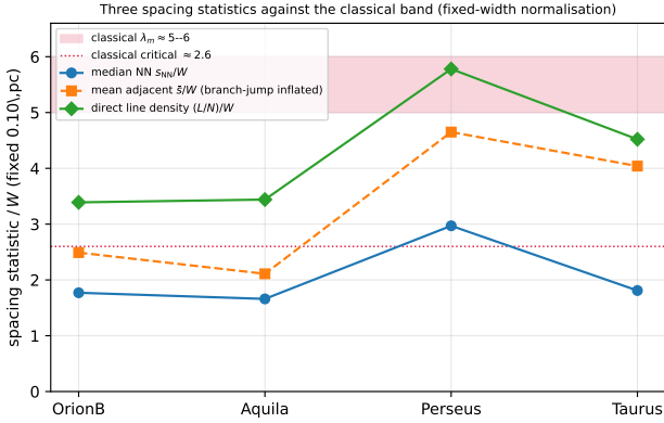
Figure 6. Three spacing statistics per cloud (single re-implementation, all normalised by the fixed 0.10 pc width so they are directly comparable), against the classical band (5–6, red; critical \approx 2.6 , dotted). The median along-skeleton ACS spacing (blue, \approx 1.7 –3.0) is sub-classical everywhere; the direct line density (L/N)/W (green, \approx 3.4 –5.8) is classical in Perseus, near-classical in Taurus, and sub-classical in Orion B and Aquila; the mean adjacent spacing (orange) lies between but is inflated by arc-length branch-jumps. The factor- \approx 2 gap between the blue and green points reflects the generic mean/median skew plus dilution by core-poor filament (a coverage effect), not small-scale clustering (Section 2.8): short adjacent spacing within core-bearing stretches, diluted by extensive core-free filament.
