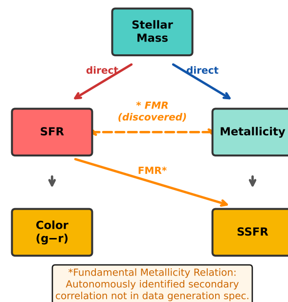
(d) Inferred Causal Structure (ASTRA autonomous discovery)
