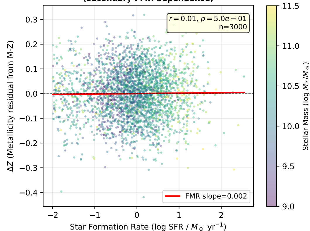
(b) SFR-driven Metallicity Scatter (secondary FMR dependence)
