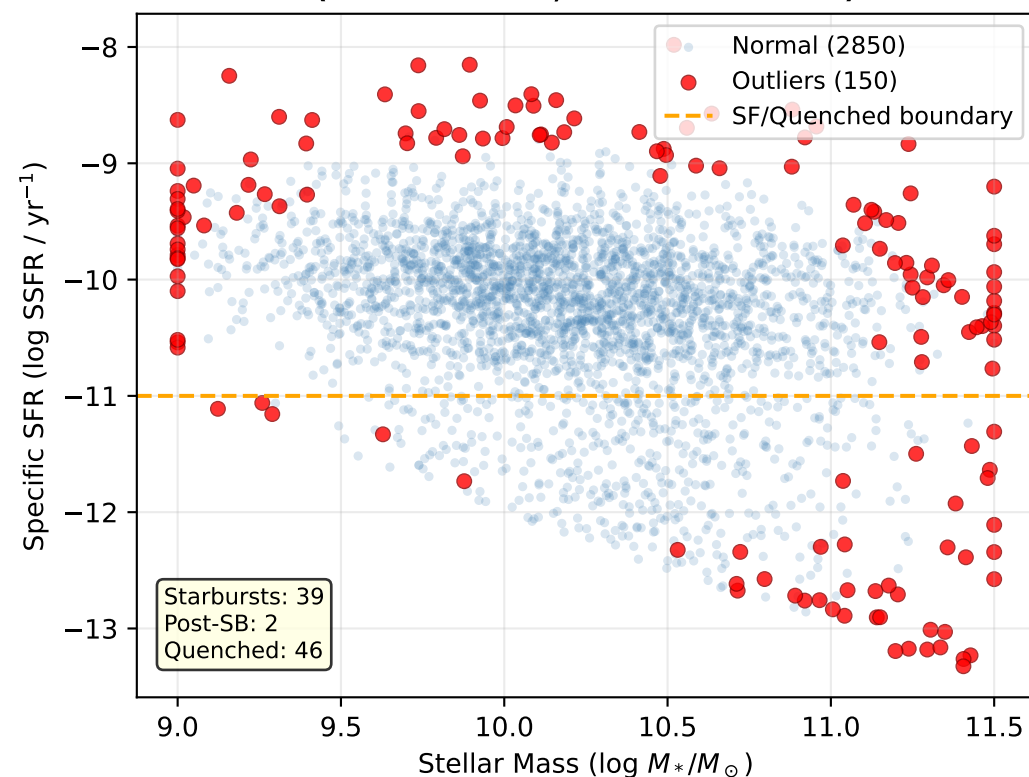
(c) Multi-dimensional Outlier Detection (IsolationForest, 5% contamination)
