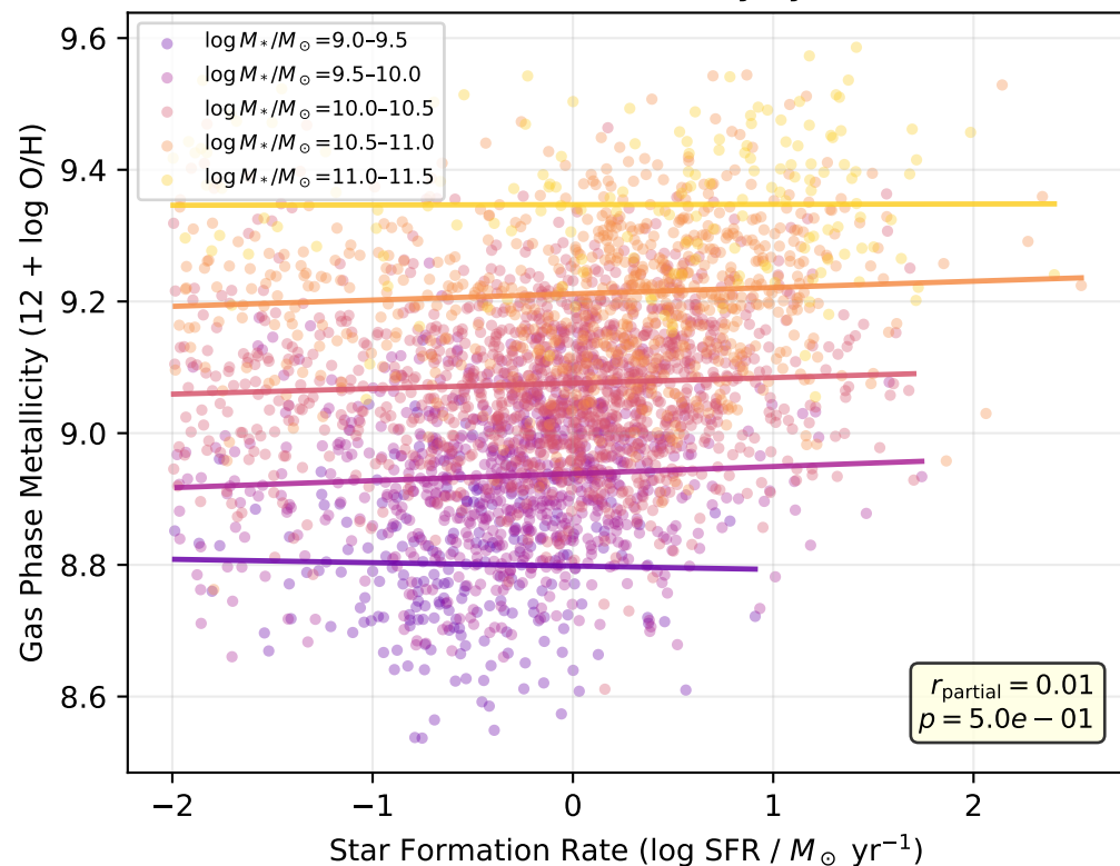
(a) Fundamental Metallicity Relation (discovered autonomously by ASTRA)
