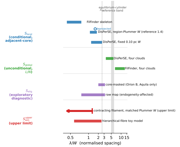
Figure 7. The full methodological envelope of \lambda/W , organised by which quantity is being measured rather than by convention alone. The four groups are the conditional adjacent-core spacing S_{\text{local}} (blue), the unconditional length per core S_{\text{global}} = (L/N)/W (green), the same restricted to fragmentation-eligible filament S_{\text{elig}} (purple); the core-masked row is fiducial, the raw-map row shows the endogeneity-affected comparison), and the simulated upper bound S_{\text{sim}}^{\text{upper}} = \lambda_{\text{turn}}/W together with the hierarchical-fibre toy model (red). Each bar spans the range across clouds and conventions; the grey band is the classical \lambda_m \approx 5\text{--}6 (Inutsuka & Miyama 1992; Fischera & Martin 2012) and the dotted line the critical \lambda_{\text{cr}} \approx 2.6 . Grouping this way makes the central point of the paper visible directly: S_{\text{local}} lies well below the classical band under every convention, S_{\text{global}} reaches it, S_{\text{elig}} falls between the two, and S_{\text{sim}}^{\text{upper}} is an upper bound that should not be read as a measured wavelength. Comparisons between groups are comparisons between different quantities and are only meaningful once that is stated (Section 2.17). The horizontal axis is symmetric-log below \lambda/W = 1 . The S_{\text{sim}}^{\text{upper}} bar is drawn with a left-pointing arrow because it is an upper limit, not a measured interval; the open marker on the S_{\text{local}} group shows where the adopted value moves if the isotropic deprojection factor of Table E2 is applied.
