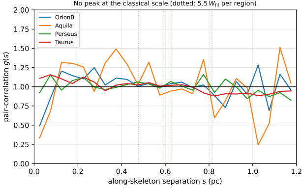
Figure 5. Along-skeleton pair-correlation function g(s) for the four primary clouds (uniform-random expectation on the matched components divided out; g = 1 is no correlation). Dotted vertical lines mark the classical scale 5.5 W_{\text{fil}} per region. No cloud shows a peak at the classical scale ( g \approx 1 there, slightly below unity in Orion B and Aquila); the only departures are a mild small-separation excess (Taurus) and weak region-envelope features near 1 pc. The classical periodic comb is therefore absent, consistent with a non-periodic, spatially inhomogeneous distribution bearing an observational small-separation deficit (Section 2.12).
