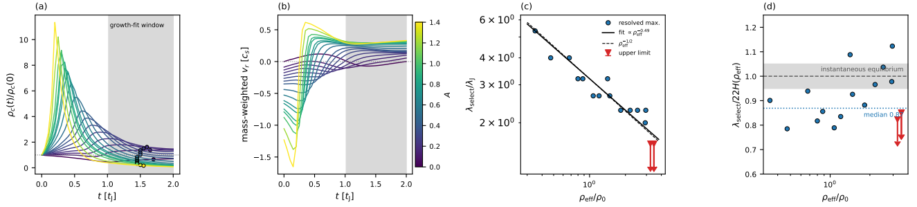
Figure 11. Contraction ladder, seventeen runs coloured by the imposed inward-velocity amplitude A . (a) Central density against time, normalised to its initial value; the shaded band is the window over which the growth rates are fitted, and the circles mark the epoch at which \rho_{\text{eff}} is evaluated. The overshoot and rebound are visible directly: a strong kick raises the density transiently and leaves the filament less dense than it started while its modes are growing. (b) Mass-weighted radial velocity within 0.6 \lambda_J of the axis, showing the same behaviour. (c) Selected scale against \rho_{\text{eff}} . Circles are runs with a resolved maximum of \Gamma ; triangles are upper limits, where \Gamma is still rising at the shortest well-resolved seeded mode. The solid line is the censored maximum-likelihood fit (Eq. 9) and the dashed line the \rho_{\text{eff}}^{-1/2} expectation. (d) The same selected scale normalised by the equilibrium result evaluated at each run’s own \rho_{\text{eff}} rather than at the initial density. Once the changing background is removed the residual shift is small: the static run sits at 1.09 and the dynamical runs have a median of 0.87, so the deficit relative to the instantaneous equilibrium expectation is of order 15 per cent, an order of magnitude smaller than the factor of three to five obtained by comparing with the initial equilibrium wavelength.
