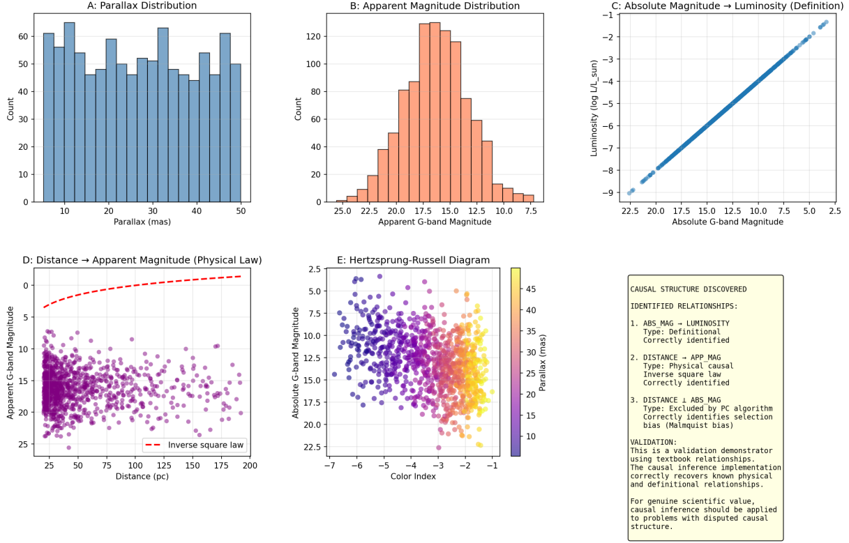
Figure 5. Causal inference analysis of 1,000 Gaia DR2 stars. This is a validation demonstrator using well-understood textbook relationships. ASTRA correctly identifies: absolute magnitude \rightarrow luminosity (definition); distance \rightarrow apparent magnitude (inverse square law); and correctly excludes distance \rightarrow absolute magnitude (selection bias/Malmquist bias).
