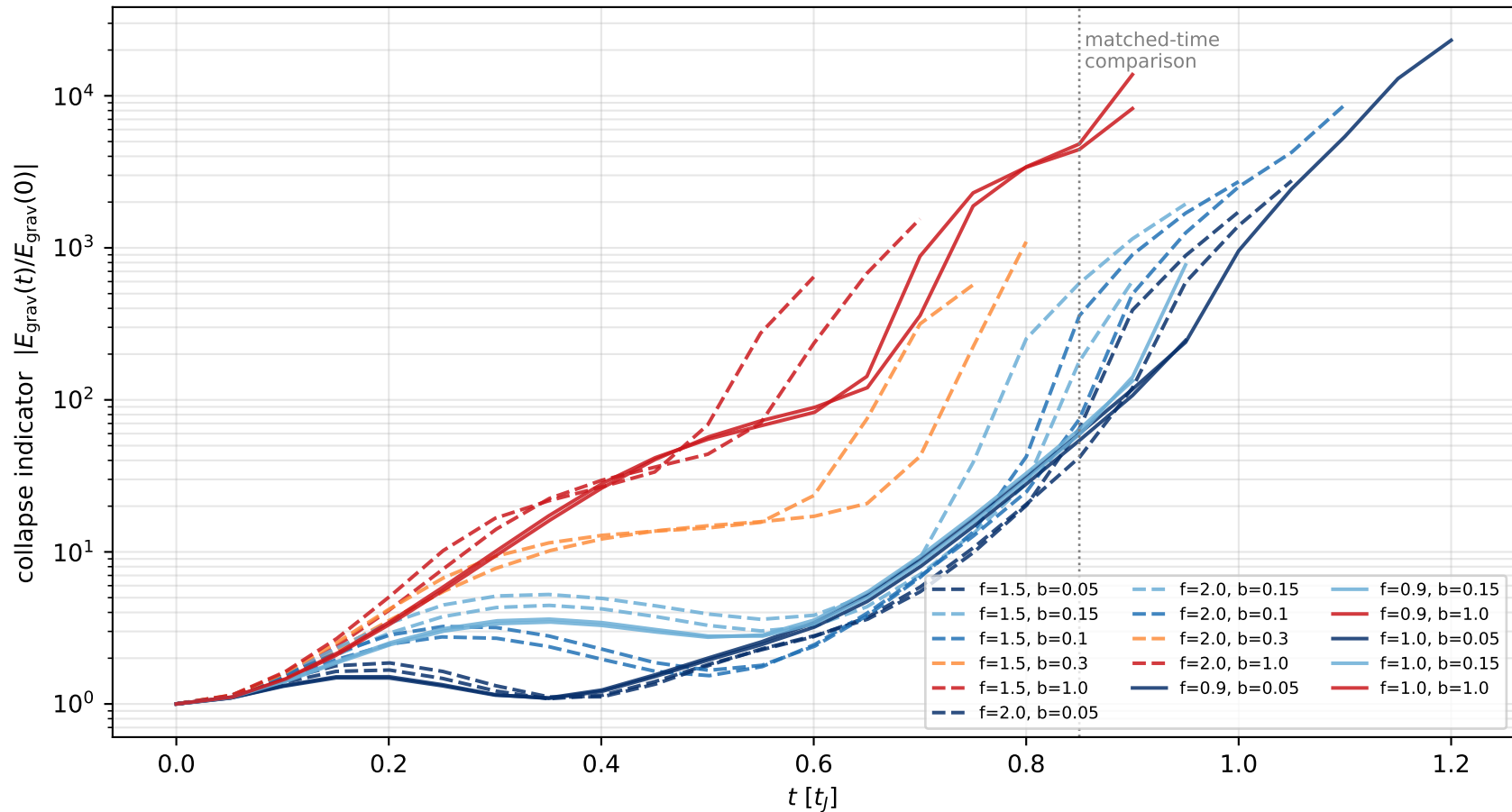
A5: radial collapse vs plasma- \beta (longitudinal B, ambient/periodic) strong field (low \beta ) strongly suppresses collapse
