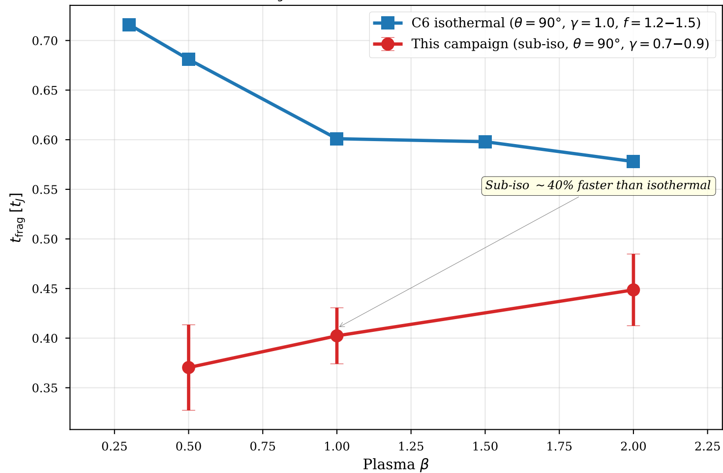
Comparison: t_{\text{frag}}(\beta) — Sub-Isothermal vs Isothermal ( \theta = 90^\circ )
