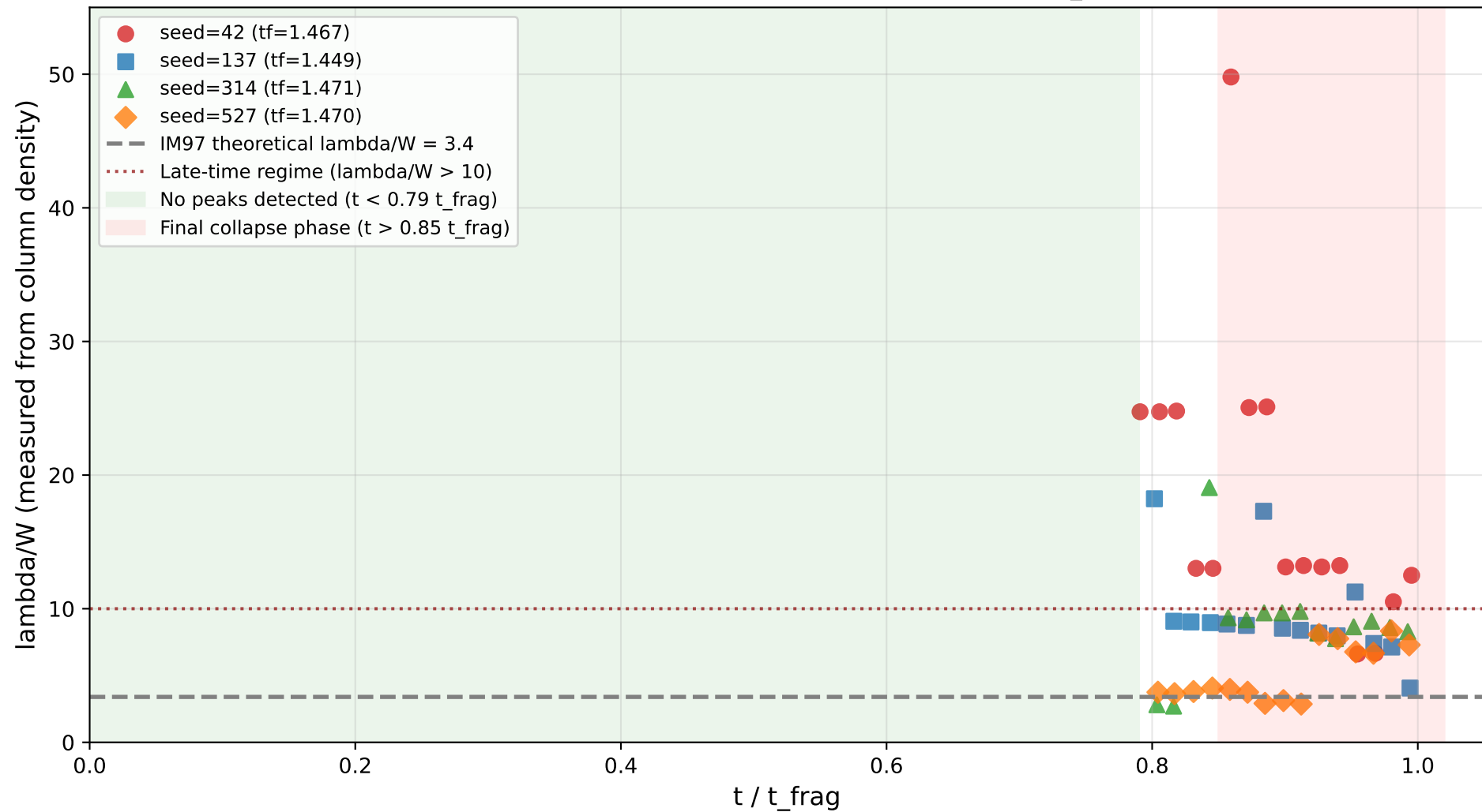
TA-1: \lambda/W Temporal Evolution -- Late-Time Sampling Bias Demonstration f=1.4 , \beta=1.0 , \theta=0 , 512 \times 64 \times 64 , L=16|J (4 seeds, \text{hdf5\_dt}=0.02 \text{ t}_J )
