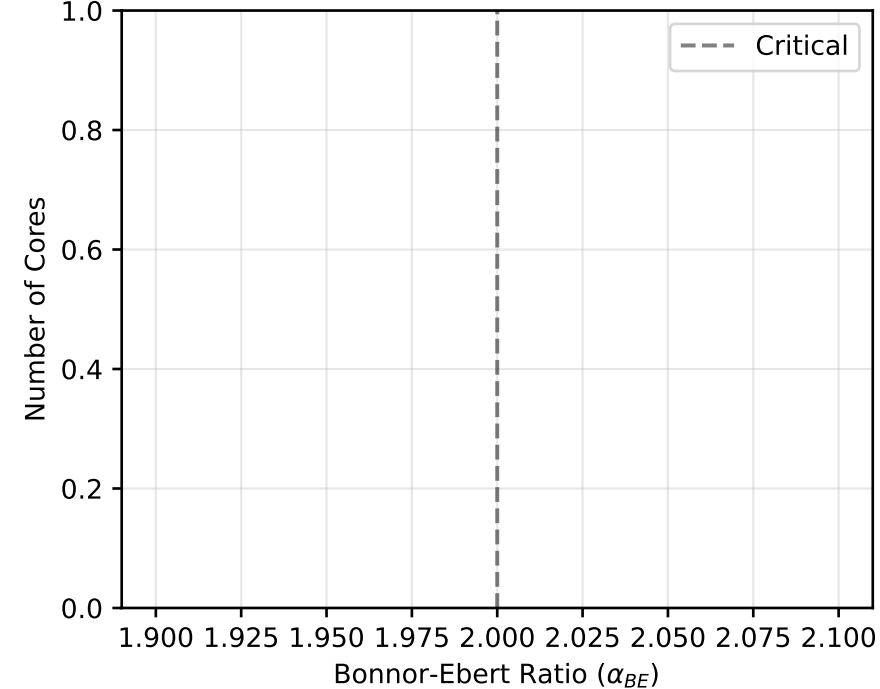
Bonnor-Ebert Ratio Distribution
