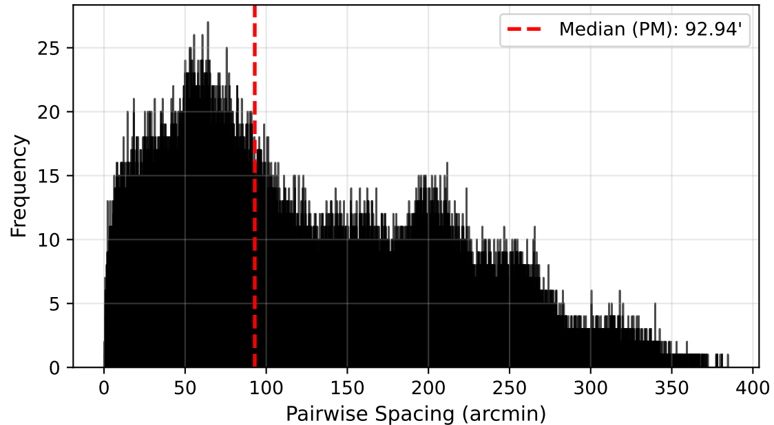
Pairwise-Median Spacing Distribution
