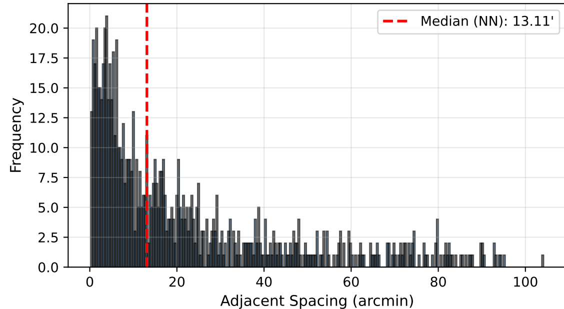
Nearest-Neighbor Spacing Distribution
