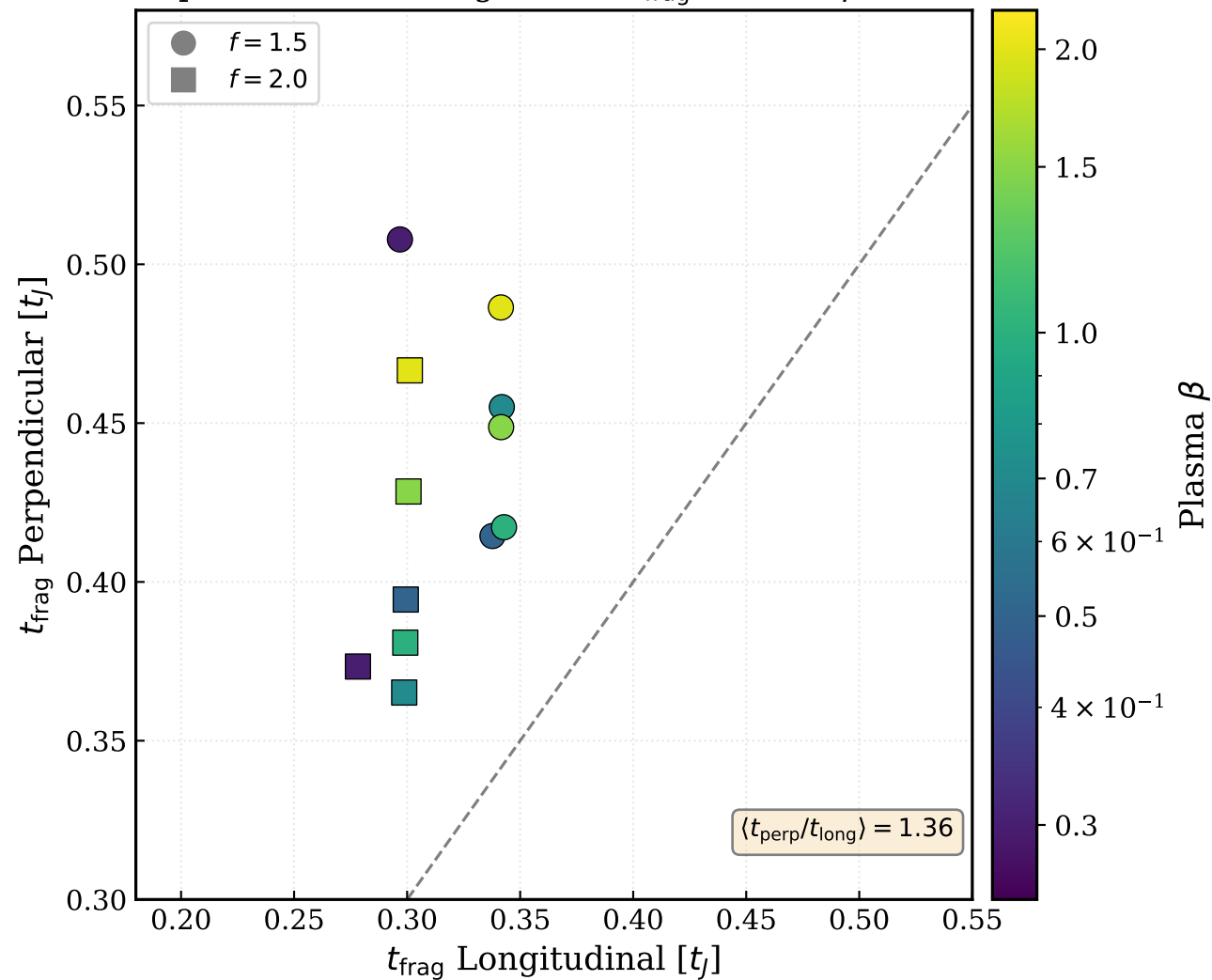
Perpendicular vs Longitudinal t_{\text{frag}} (same f , \beta , M = 1 )
