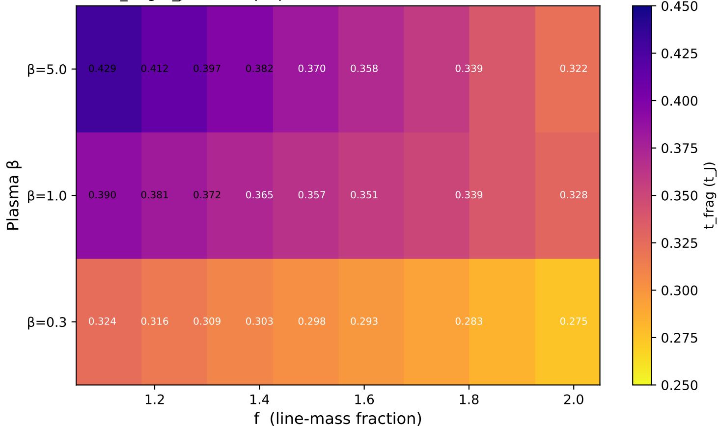
t_frag [t_J] \theta=90^\circ perpendicular field, M=1, mean of 2 seeds
