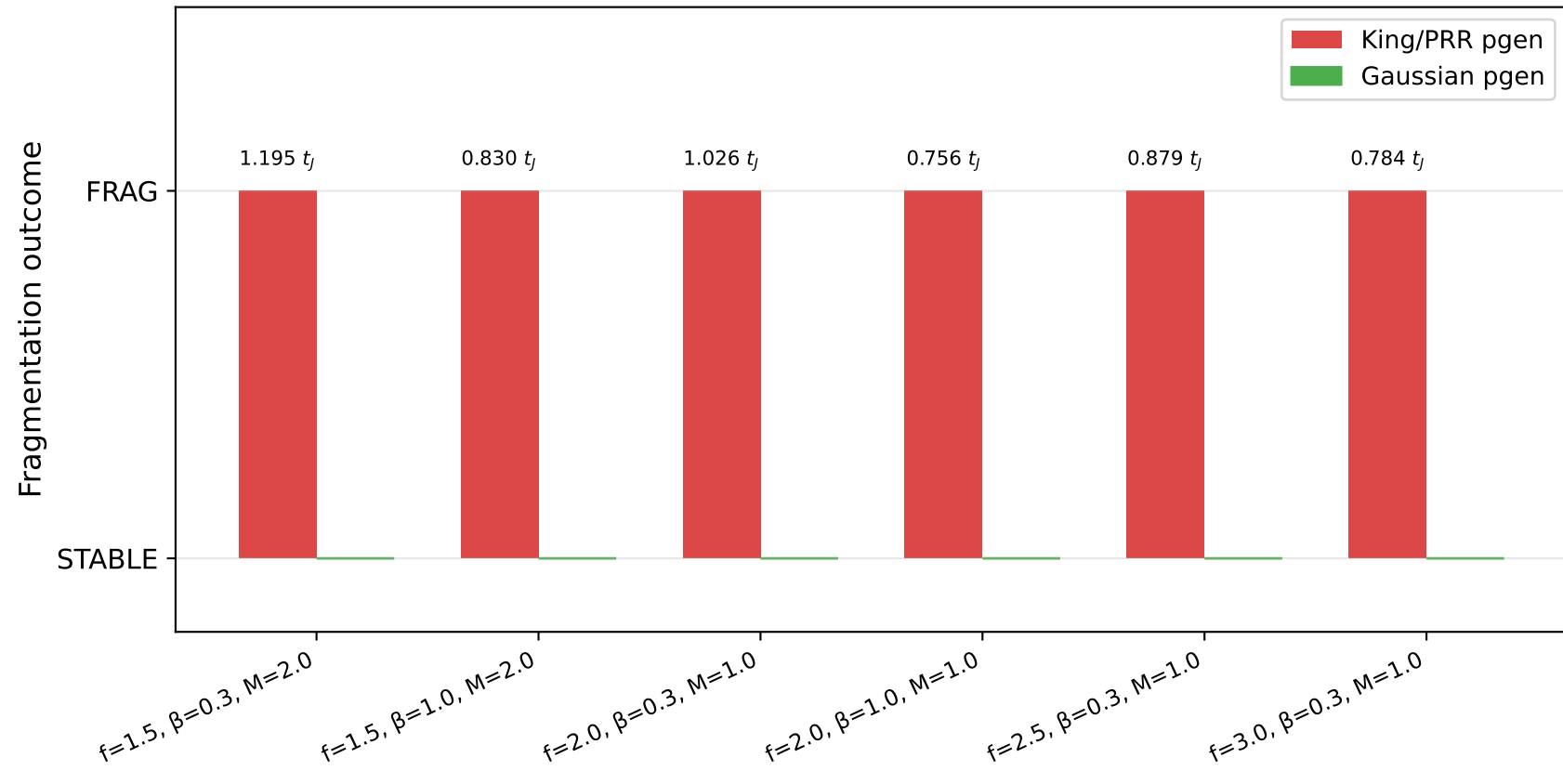
IC-Sensitivity: King/PRR vs Gaussian pgen Same ( f , \beta , M , resolution) — matched pairs
